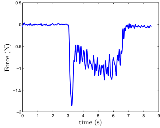
(b) Contact forces during sponging action measured on a flat panel coupled to a force/torque sensor.
