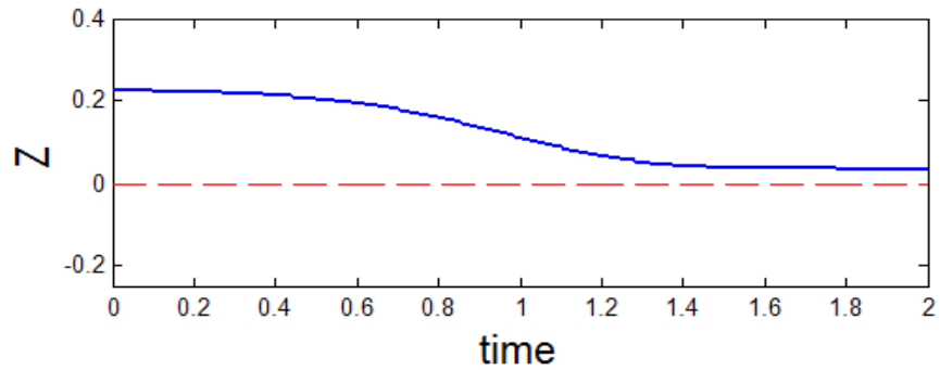
(b) Arm tip vertical position (in meters) when minimum jerk trajectories are used to move between desired joint angles of the simulated inflatable arm
