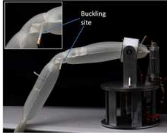
(b) Failure due to buckling of the inflatable joint. The inset figure shows buckling on the lower side of the inflatable joint.
