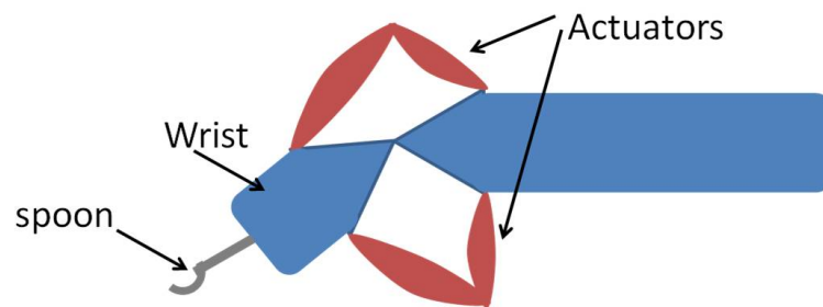
(a) Schematic showing wrist and inflatable variable stiffness actuator (IVSA) arrangement
