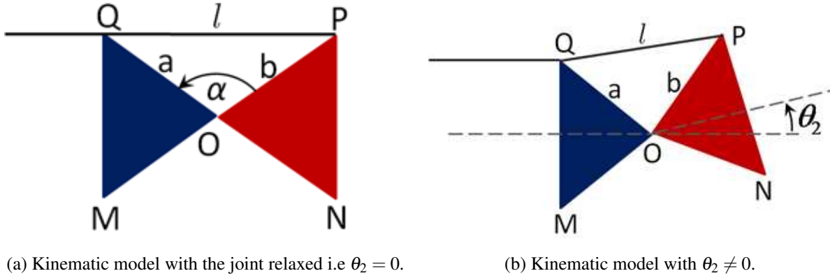
Figure 4.13: Rigid body kinematic model of joint 2 using two rigid bodies O-Q-M and O-N-P connected at O via a revolute joint. Vertex Q represents the last point on link 1 through which the tendon is constrained to pass through while vertex P represents the tendon attachment location on link 2. \alpha is the angle between O-Q and O-P when \theta_2 = 0 . a and b are the lengths of O-Q and O-P respectively, l is the length of the tendon between vertex Q and P.
