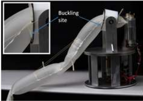
(a) Failure due to buckling of the inflatable link 1.
