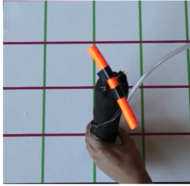
(b) Inflated configuration
