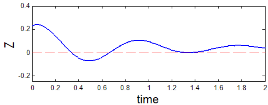
(a) Arm tip vertical position (in meters) when only PD control + gravity compensation is used to move between desired joint angles of the simulated inflatable arm
