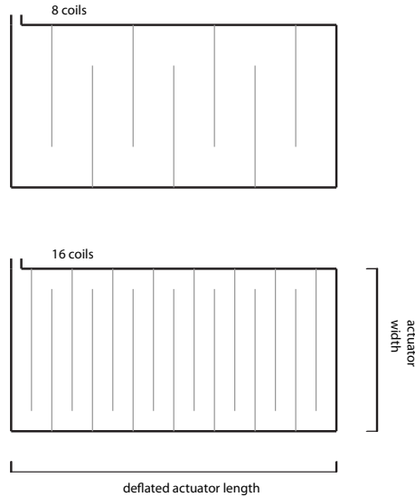
Figure 7.7: Peano actuators with different number of tubes or coils. For both the actuators shown here the actuator length contraction is identical.
