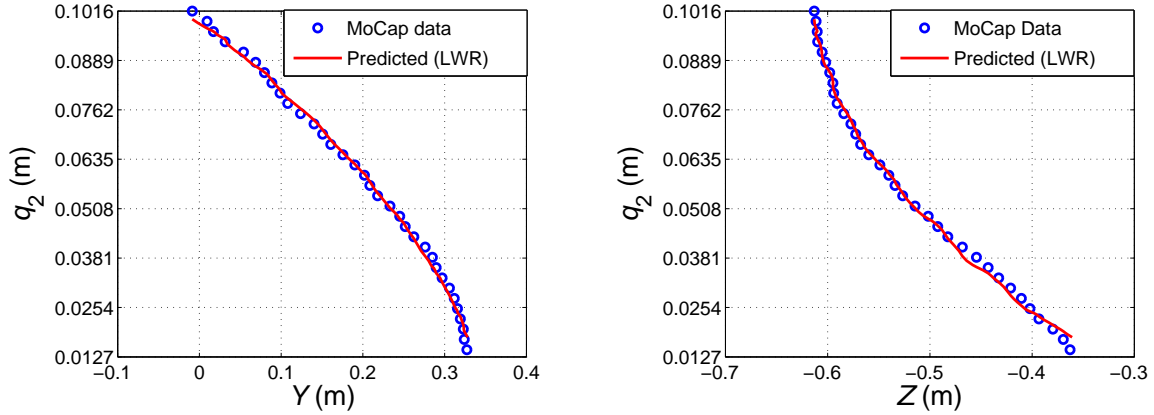
(a) Predicted and actual position values of the second actuator q_2 plotted with Y coordinate of the arm end
