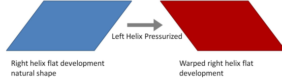
Figure 7.4: Flat development of helix during actuator motion
