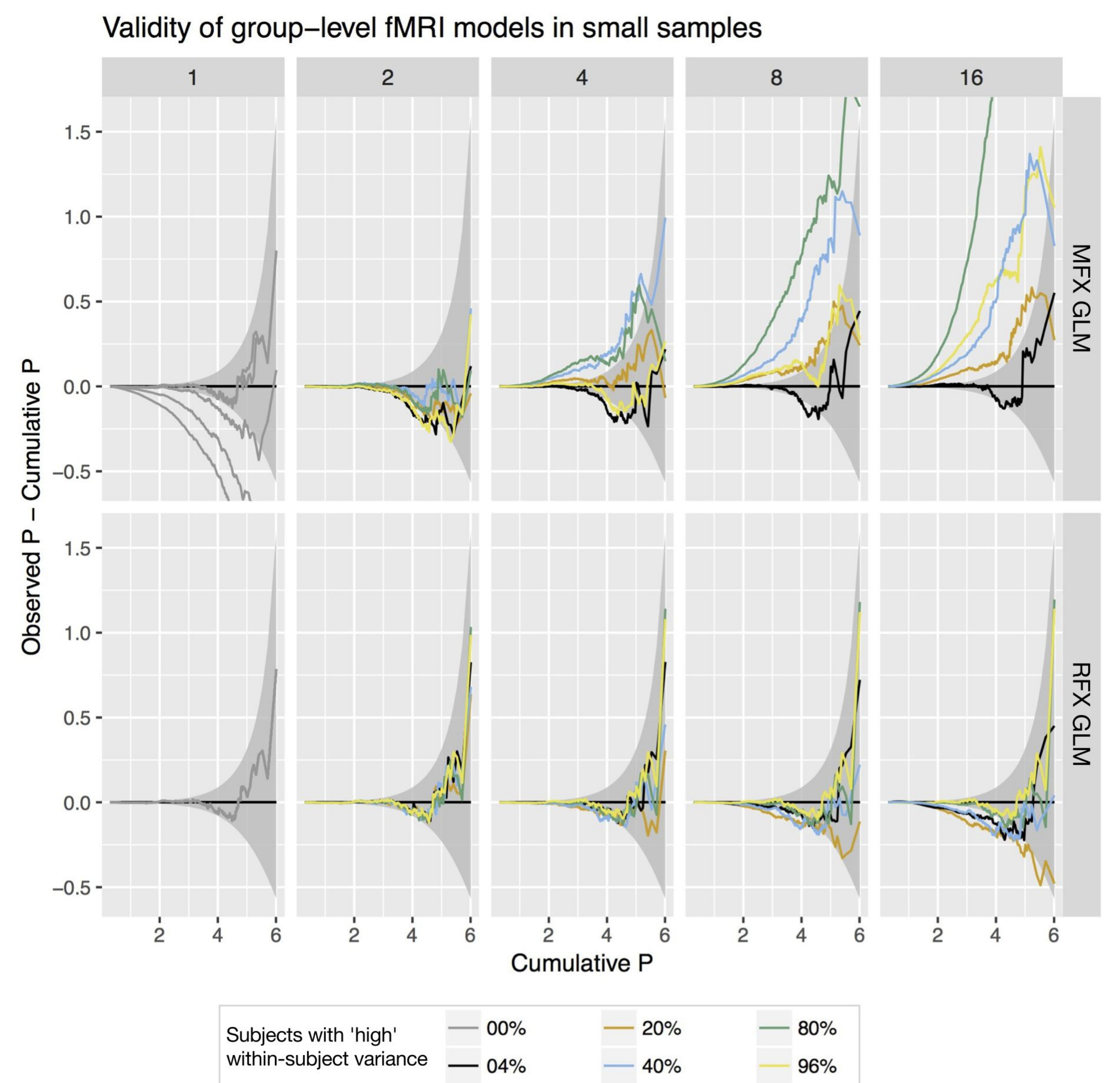
Fig. 1. Deviation of observed from theoretical P-values (difference of observed and Monte Carlo ('true') -log 10 p-value distributions) for one-sample tests in the presence of varying percentages of subjects with outlying within-subject variances, high-variance factor 2, 4, 8 or 16, (columns), MFX GLM and RFX GLM (rows). Y-axis is the observed cumulative probability minus Monte Carlo cumulative probability for a given (X-axis) -log 10 p-value; positive deflections correspond to inflated false positive risk.
