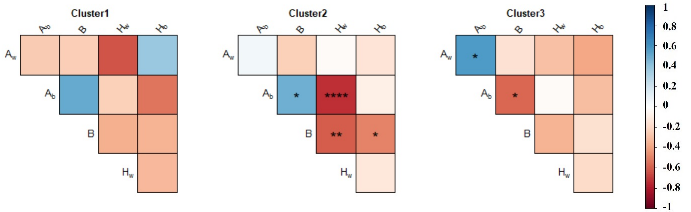
Figure S7 Pearson's correlation test performed to investigate the intra-cluster correlations at the trait level: for each cluster, the figure shows the correlation between variances of the genetic effects. * significant at p < 0.05 ; ** significant at p < 5 \cdot 10^{-3} ; *** significant at p < 5 \cdot 10^{-4} ; **** significant at p < 5 \cdot 10^{-5} . No symbol: not significant.
