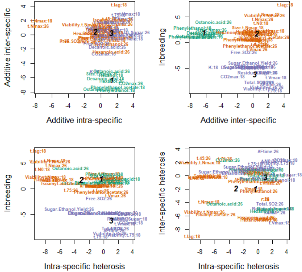
Figure S6 Life-history and fermentation traits profiles. Traits are identified by their label, color combinations identify the clusters obtained by their classification based on a Gaussian Mixture model.
