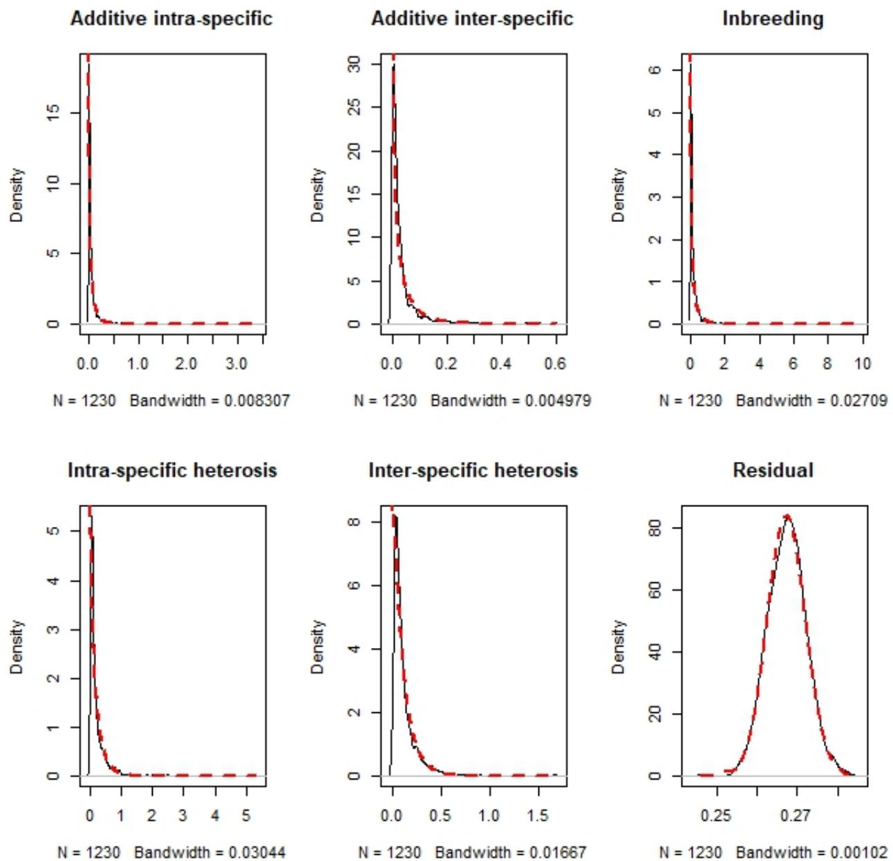
Figure S1 Density of the variance components estimated by the hglm algorithm for the 1230 proteins. Red dashed lines represent the fitted distributions used to simulate and test parameter inference of the proposed model.
