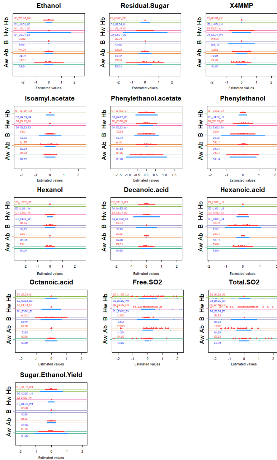
Figure S12 Interval plots. For each fermentation and life-history trait we plot the Best Linear Unbiased Predictors of the random genetic effects estimated through the decomposition of our diallel design. The random genetic effect estimates, namely \hat{A}_w , \hat{A}_b , \hat{B} , \hat{H}_w , \hat{H}_b are plotted in blue (18°C), or in red (26°C). Horizontal bars are added to show, for each parameter, the region of highest density that covers nearly 95% ( \sim \pm 2\hat{\sigma}_g ) of the parameter density. On the left hand-side of each plot we list, for each genetic effect, the strains which have the lowest and the greatest (ii) of the respective genetic effect. The plot shows that: (i) genetic effects differ in a large extent between the two temperatures; (ii) additive and heterosis effects depend on the type of cross in which a line is involved (intra- or inter-specific); (iii) for some traits, genetic variances are strongly influenced by a particular hybrid combination.
