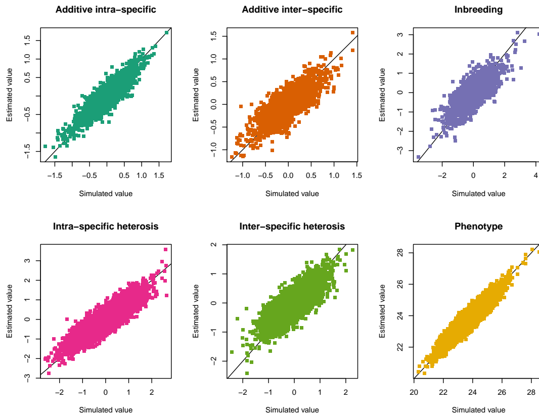
Figure S2 Fitted Best Linear Unbiased Predictors of the random effects parameters and predicted phenotypic value plotted against the simulated genetic parameters and the simulated phenotypic value. Fixed the number of parental strains and the number of individuals of each species, we performed the simulation 1000 times. Here, we show the case of eleven parents, with 7 belonging to one specie and 4 to the other.
