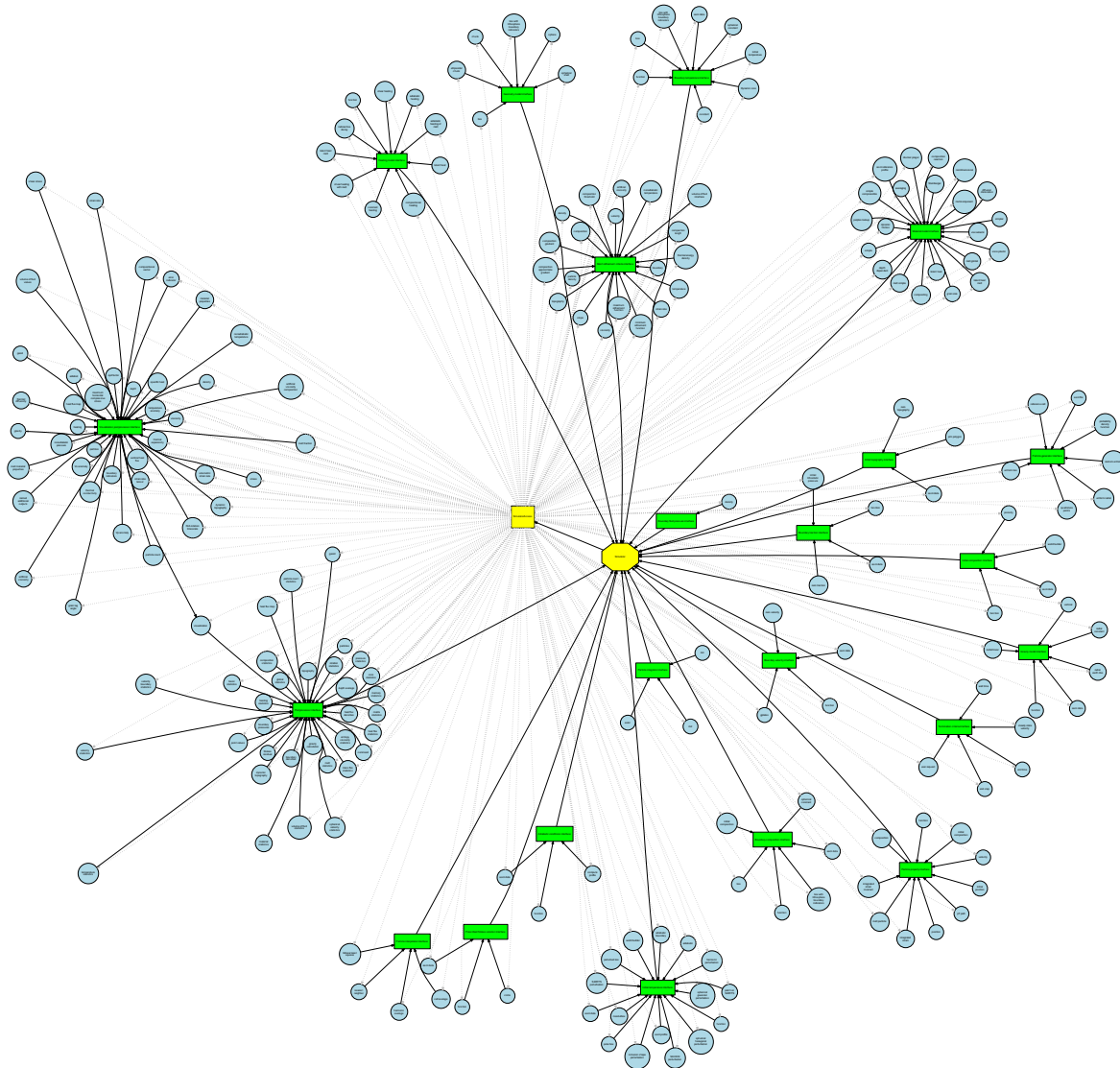
Figure 103: The graph of all current plugins of ASPECT. The yellow octagon and square represent the Simulator and SimulatorAccess classes. The green boxes are interface classes for everything that can be changed by plugins. Blue circles correspond to plugins that implement particular behavior. The graph is of course too large to allow reading individual plugin names (unless you zoom far into the page), but is intended to illustrate the architecture of ASPECT.
