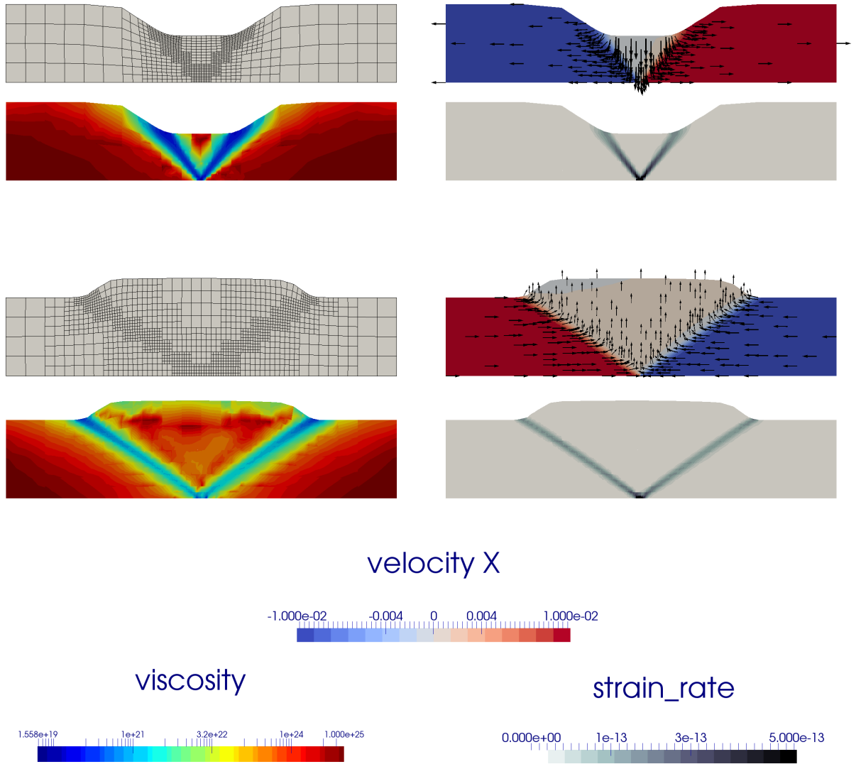
Figure 53: Finite element mesh, velocity, viscosity and strain rate fields in the case of extensional boundary conditions (top) and compressive boundary conditions (bottom) at t=500\text{kyr} .
