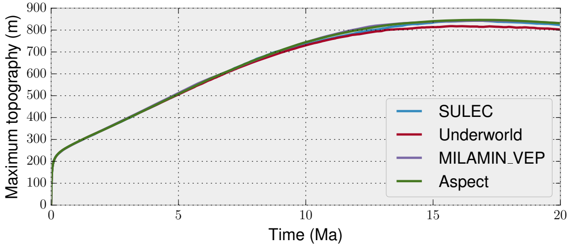
Figure 94: Evolution of topography for the dynamic topography benchmark. The maximum topography is shown as a function of time, for ASPECT as well as for several other codes participating in the benchmark. This benchmark shows considerably more scatter between the codes.
