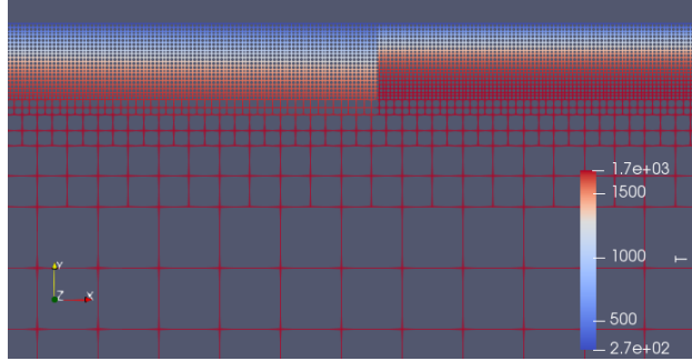
Figure 36: Initial temperature condition for the lazy-expression syntax cookbook within the region where the two plates meet. The wireframe shows the element size refinement.
