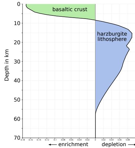
Figure 64: Vertical profile through the model domain at a distance of 80 km from the ridge axis at the end of the model run, showing the distribution of depletion and enrichment as indicated by the peridotite field.
