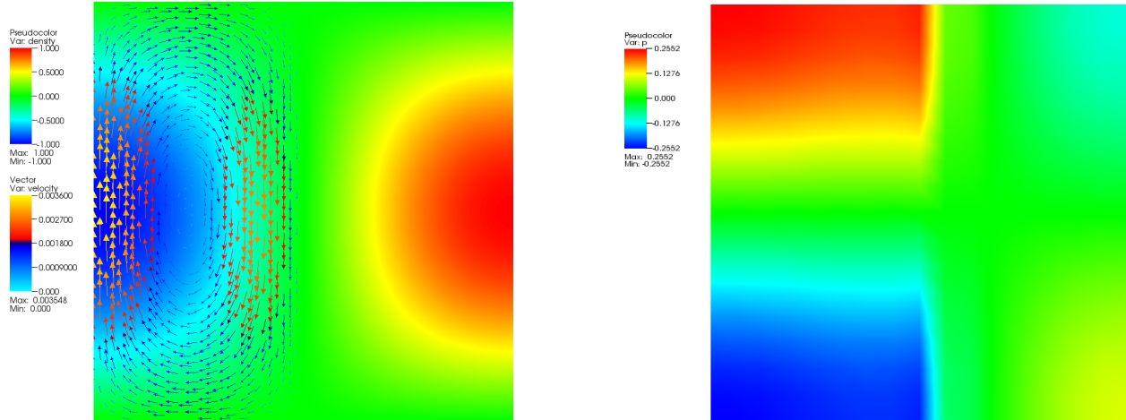
Figure 76: SolCx Stokes benchmark. Left: The density perturbation field and overlaid to it some velocity vectors. The viscosity is very large in the right hand, leading to a stagnant flow in this region. Right: The pressure on a relatively coarse mesh, showing the internal layer along the line where the viscosity jumps.
