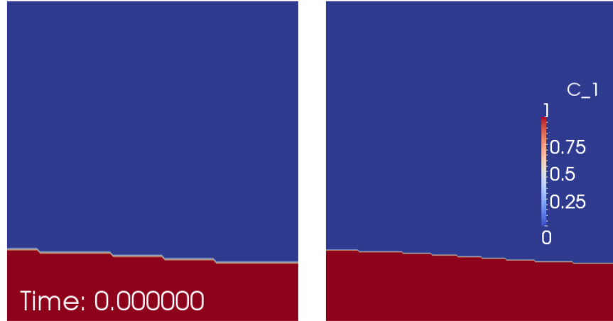
Figure 69: Van Keken benchmark with discontinuous initial conditions for the compositional field: Initial compositional field interpolated onto a 32 \times 32 (left) and 64 \times 64 finite element mesh (right).
