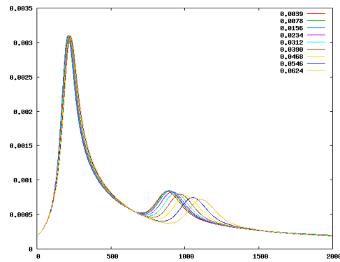
Figure 72: Van Keken benchmark with smoothed initial conditions for the compositional field using 7 global refinements for different smoothing parameters. Number of the time step is shown on the x-axis, while root mean square velocity is shown on the y-axis.
