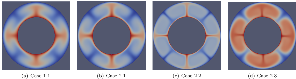
Figure 89: Davies et al. benchmarks: Final steady state temperature fields for the 2D cylindrical benchmark cases.
