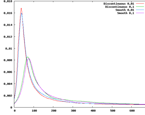
Figure 75: Van Keken benchmark: Evolution of the root mean square velocity as a function of time for different viscosity contrast proportions (0.1/0.01) for both discontinuous and smooth models.
