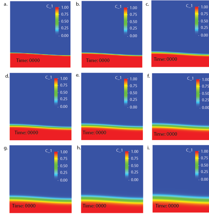
Figure 71: Van Keken Benchmark using smoothed out interface at 7 global refinements: compositional field at time t = 0 using smoothing parameter size: a) 0.0039, b) 0.0078, c) 0.0156, d) 0.0234, e) 0.0312, f) 0.0390, g) 0.0468, h) 0.0546, i) 0.0624.
