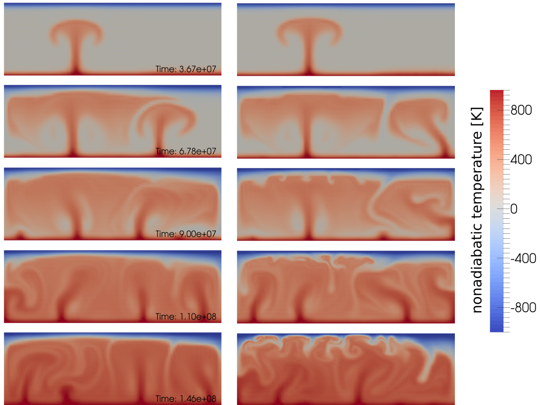
Figure 62: Evolution of the model without (left) and with (right) melt migration.
