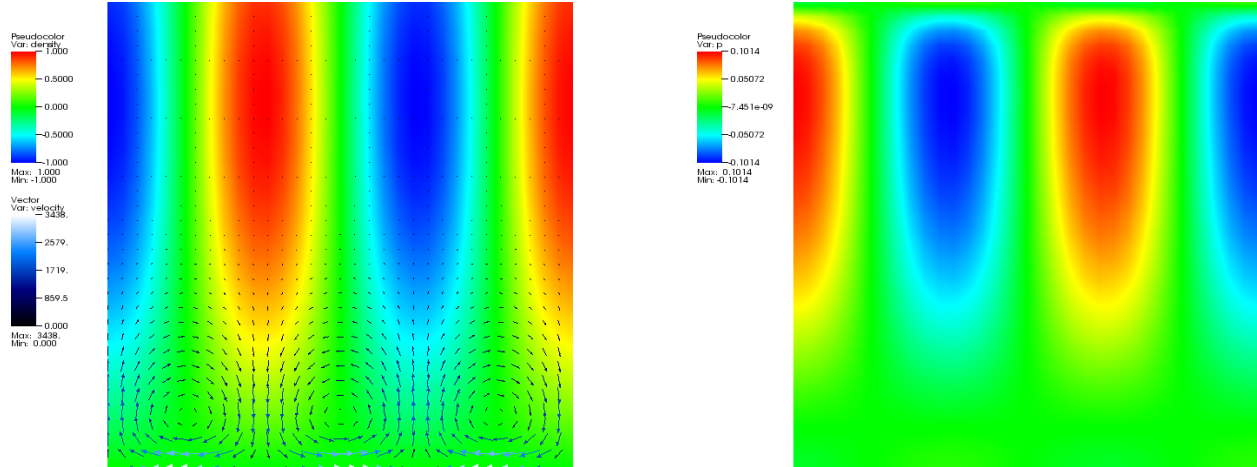
Figure 77: SolKz Stokes benchmark. Left: The density perturbation field and overlaid to it some velocity vectors. The viscosity grows exponentially in the vertical direction, leading to small velocities at the top despite the large density variations. Right: The pressure.
