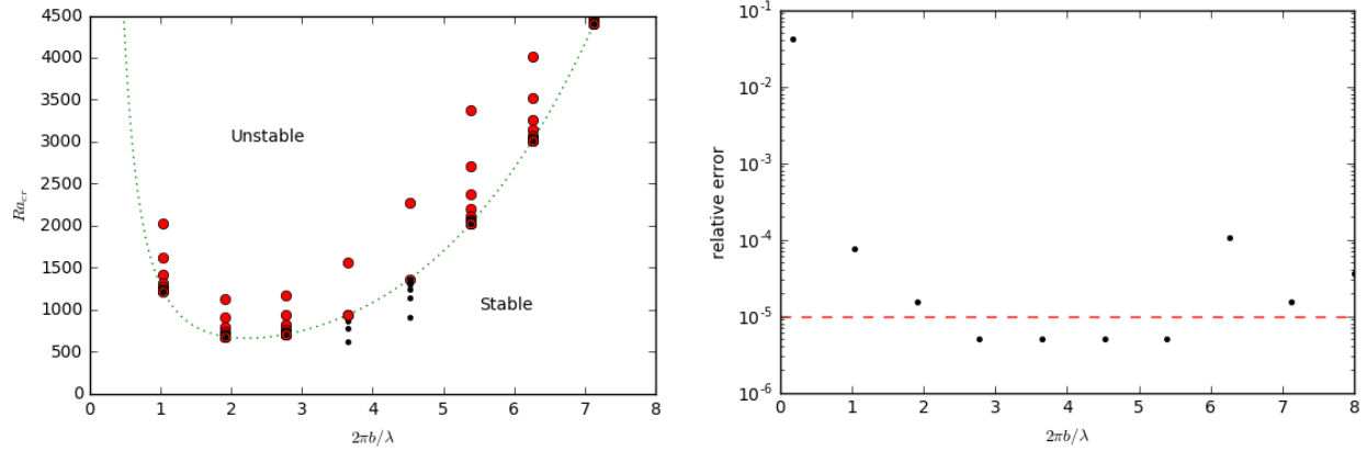
Figure 66: Left: Comparison of numerically-determined and theoretical values for Ra_c . Red circles indicate numerical simulations unstable to convection, black circles indicate simulations that are stable. The green dashed curve indicates the theoretical prediction. Right: Relative error in determination of Ra_c . The dashed red line indicates the error tolerance used in bisection procedure.
