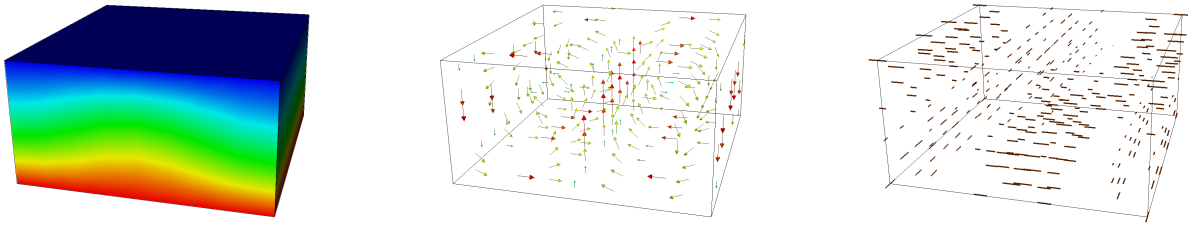
Figure 104: Illustration of the ‘maximum horizontal compressive stress’ visualization plugin. The left figure shows a ridge-like temperature anomaly. Together with no-slip boundary along all six boundaries, this results in two convection rolls (center). The maximal horizontal compressive strength at the bottom center of the domain is perpendicular to the ridge because the flow comes together there from the left and right, yielding a compressive force in left-right direction. At the top of the model, the flow separates outward, leading to a negative compressive stress in left-right direction; because there is no flow in front-back direction, the compressive strength in front-back direction is zero, making the along-ridge direction the dominant one. At the center of the convection rolls, both horizontal directions yield the same stress; the plugin therefore chooses an essentially arbitrary horizontal vector, but then uses a zero magnitude given that the difference between the maximal and minimal horizontal stress is zero at these points.
