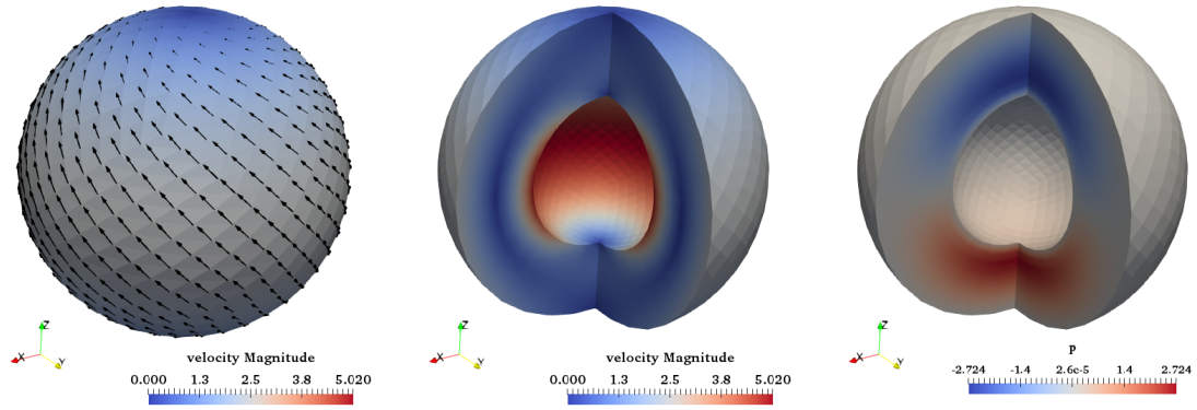
Figure 81: Velocity and pressure fields for the hollow sphere benchmark.
