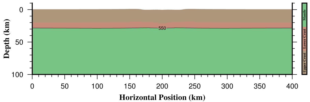
Figure 57: Compositional field after 5e6 years of extension. The black line marks the 550\text{ }^{\circ}C isotherm.
