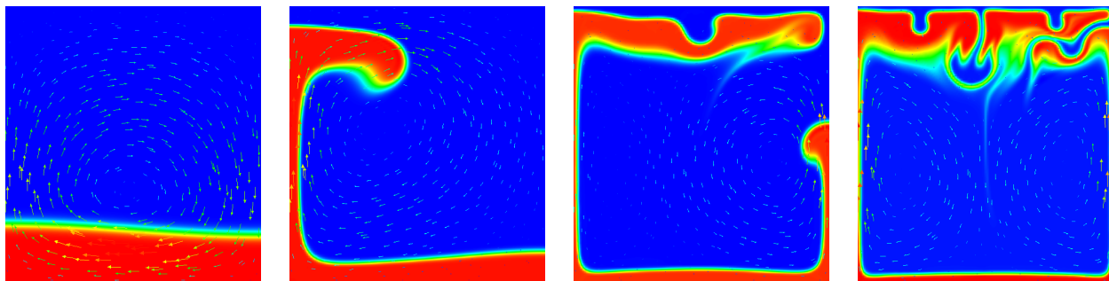
Figure 67: Van Keken benchmark (using a smoothed out interface, see the main text): Compositional field at times t = 0, 300, 900, 1800 .
