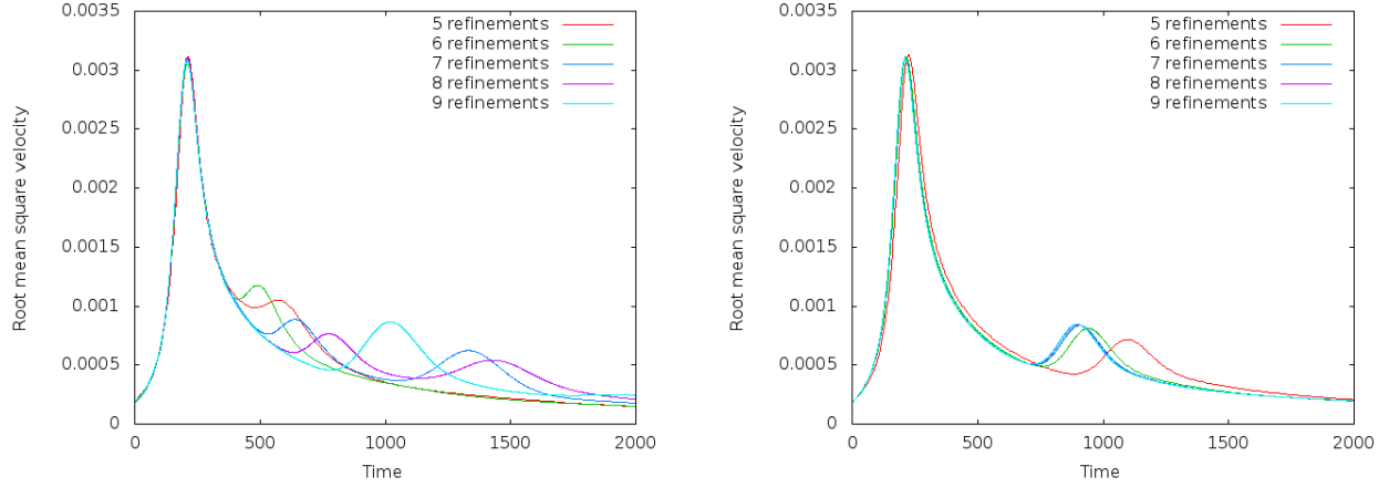
Figure 68: Van Keken benchmark with discontinuous (left) and smoothed, continuous (right) initial conditions for the compositional field: Evolution of the root mean square velocity \left(\frac{1}{|\Omega|} \int_{\Omega} |\mathbf{u}(\mathbf{x}, t)|^2 dx\right)^{1/2} as a function of time for different numbers of global mesh refinements. 5 global refinements correspond to a 32 \times 32 mesh, 9 refinements to a 512 \times 512 mesh.
