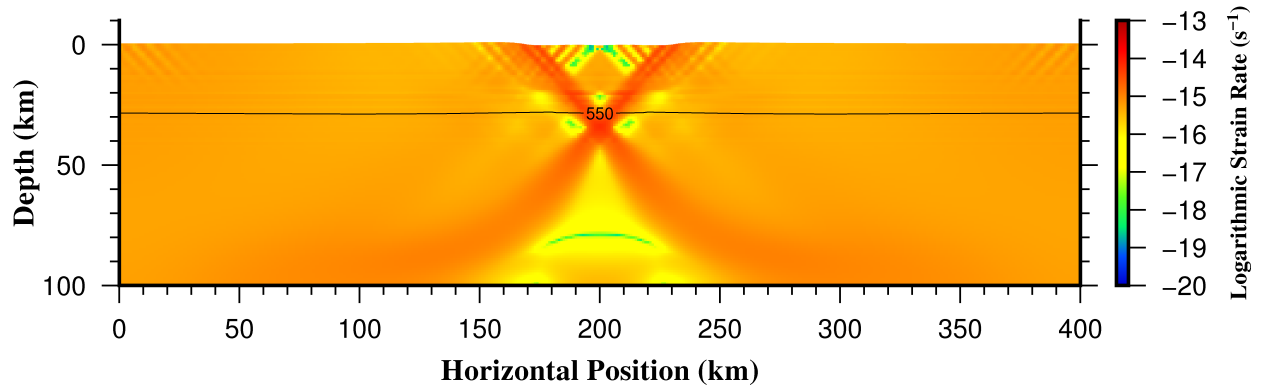
Figure 56: Strain rate ( s^{-1} ) after 5e6 years of extension. The black line marks the 550\text{ }^{\circ}C isotherm.
