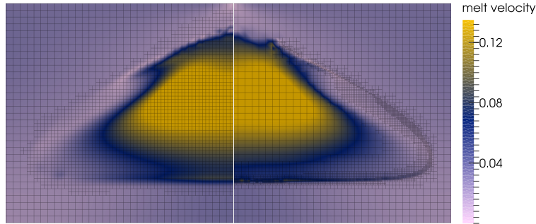
Figure 65: Mesh after a time of 3.6 million years for a model using the composition threshold refinement strategy (left) and the compaction length refinement strategy (right) Background colors indicate the melt velocity. Its sharp gradients at the interface between regions with and without melt can only be resolved using the compaction length refinement strategy.
