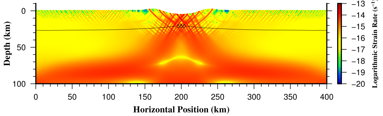
Figure 58: Strain rate ( s^{-1} ) after 10e6 years of extension. The black line marks the 550 °C isotherm. The numerical resolution (1 km) is double that of the previous model.
