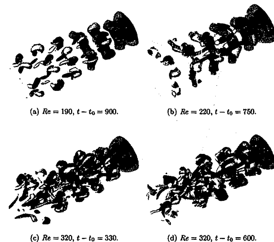
FIGURE 6.8: Isosurface plots of the saturated wake structures in the flow past a ring with Ar = 5 at various Reynolds numbers. The azimuthal domain size is \lambda_d = L_0 \approx 4d . Blue and yellow contours show positive and negative streamwise vorticity, highlighting non-axisymmetric wake structures. The translucent red isosurface represents a pressure contour to highlight the position of the rollers which comprise the vortex street. The ring is coloured green, and flow is from top right to bottom left in each frame.
