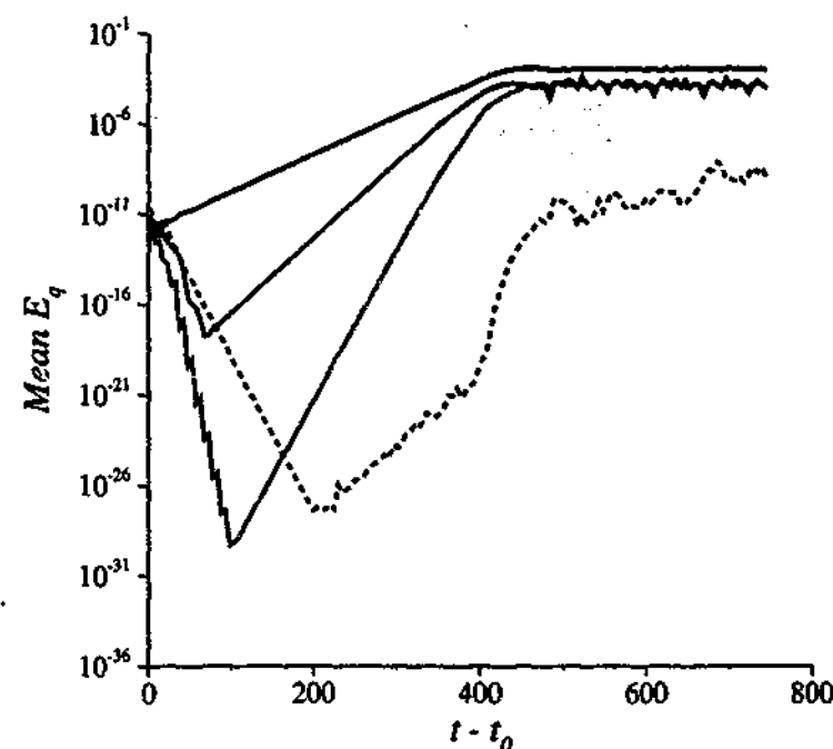
FIGURE 6.17: Evolution of the mean kinetic energy per period ( E_q ) for each azimuthal mode in the flow past a ring with Ar = 20 at Re = 205 . Axes and lines are as per figure 6.1.
