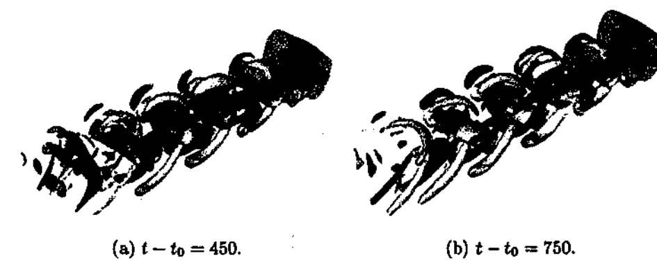
FIGURE 6.18: Isosurface plots of the saturated wake structures in the flow past a ring with Ar = 20 at Re = 205 , at the initial saturation point (a), and after the evolution of the fundamental azimuthal mode (b). The azimuthal domain size and contour shading are as per figure 6.8.
