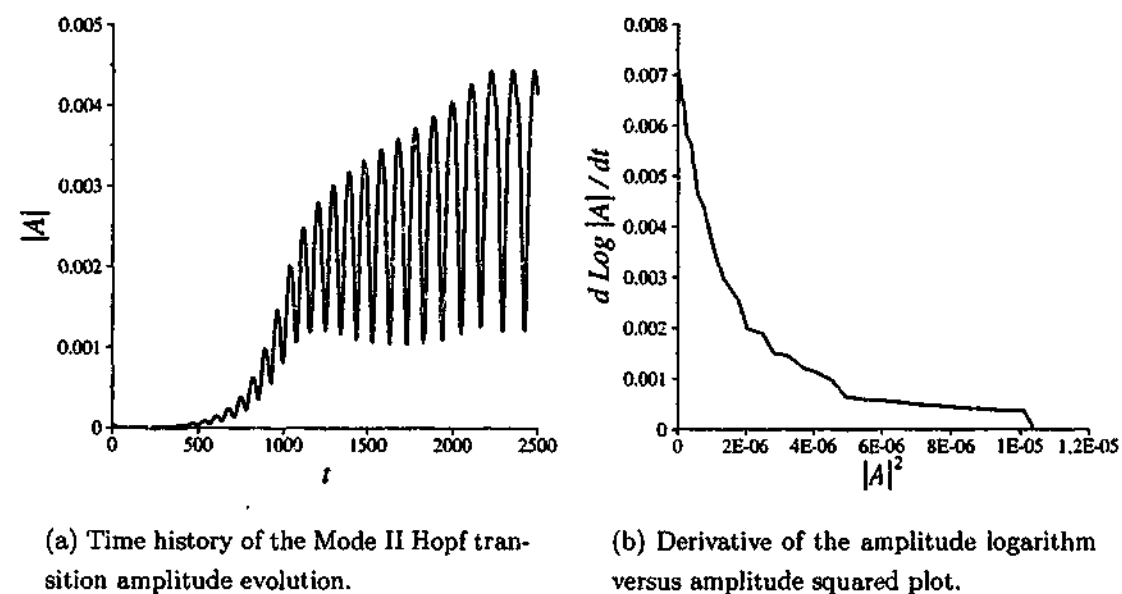
FIGURE 5.9: Plots used to determine the coefficients of the Landau model for the Mode II Hopf transition in the flow past a ring with Ar = 1.6 at Re = 98 . In (b), the negative slope near the y -axis indicate that the transition is supercritical.
