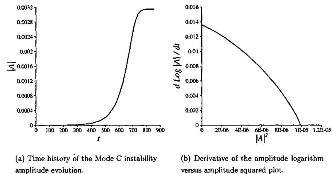
FIGURE 5.19: Plots used to determine the coefficients of the Landau model for the Mode C transition in the flow past a ring with Ar = 5 at Re = 170 . In (b), the negative slope near the y -axis indicates that the transition is supercritical.
