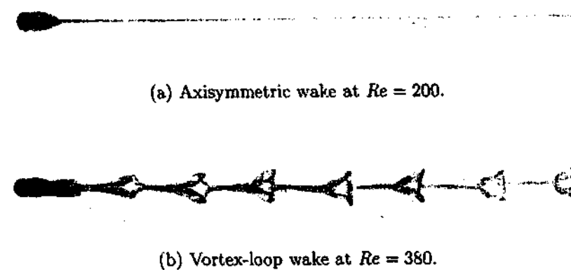
FIGURE 1.3: Reproductions of dye visualisation photographs from Magarvey & Bishop (1961b), which show spherical droplets falling through a liquid. For illustrative purposes, the flow is presented here from left to right.
