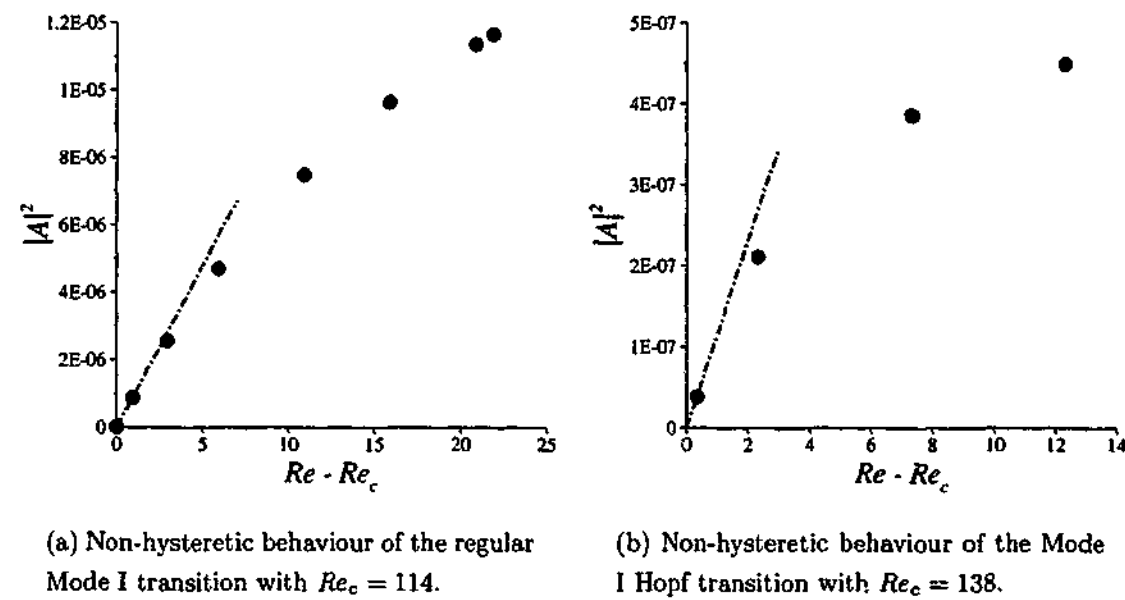
FIGURE 5.4: Plots of |A|^2 with Re - Re_c in the vicinity of the transition for both the regular (a) and Hopf (b) transitions in the flow past a ring with Ar = 0.6 in the Mode I flow regime. The dots represent the measured amplitudes, and the lines provide a linear fit to the data through Re - Re_c = 0 .
