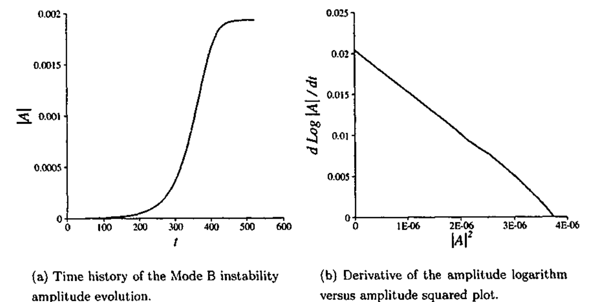
FIGURE 5.28: Plots used to determine the coefficients of the Landau model for the Mode B transition in the flow past a ring with Ar = 10 at Re = 275 . In (b), the linear profile and negative slope near the y -axis indicate that the transition is supercritical.
