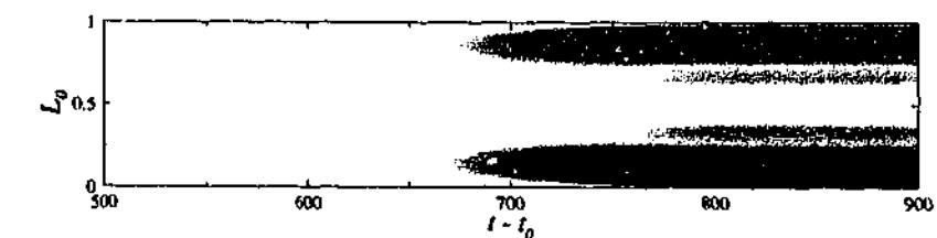
(a) Re = 205 .
