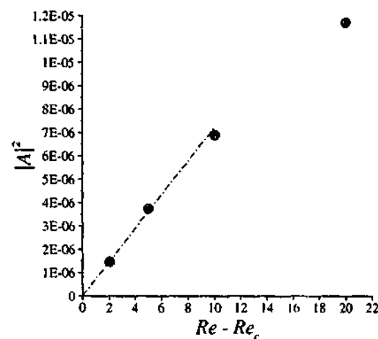
(c) Non-hysteretic behaviour of a pure Mode B instability with Re_c = 270.0 .
