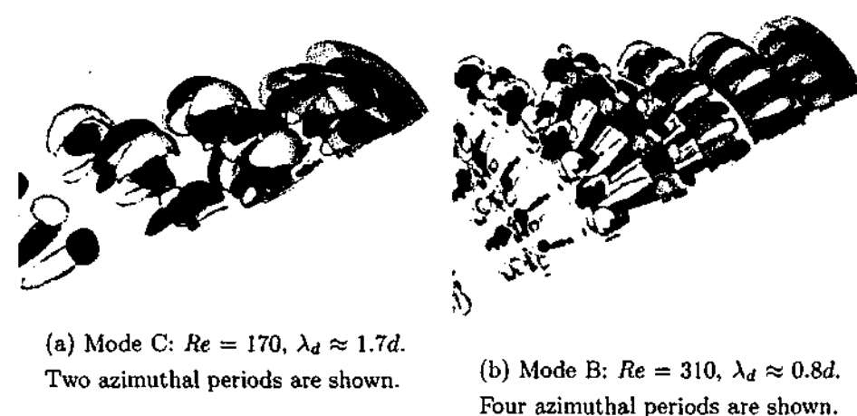
FIGURE 5.18: Vortex structure of the saturated non-axisymmetric wakes of a ring with Ar = 5 following the Mode C (a) and Mode B (b) instabilities. Blue and yellow contours represent positive and negative streamwise vorticity, respectively. A pressure level of -0.1 is represented by a translucent red isosurface, which shows the rollers in the vortex street. The ring is coloured green, and is located at the upper right corner of each frame, with the flow direction towards the lower left corner.
