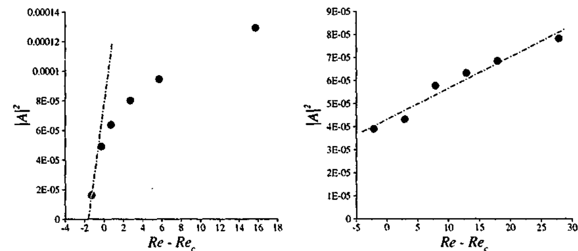
(a) Weakly hysteretic behaviour of a pure Mode A instability with Re_c = 194.3 .
