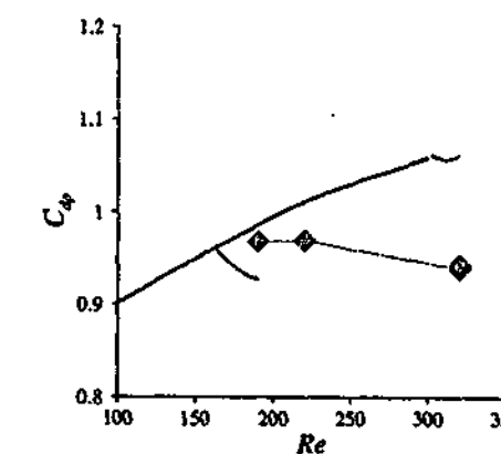
(b) Pressure component ( C_{dp} ).
