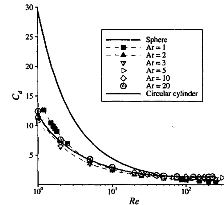
(a) C_d versus \log Re .
