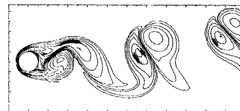
(e) t = 1.0T .
