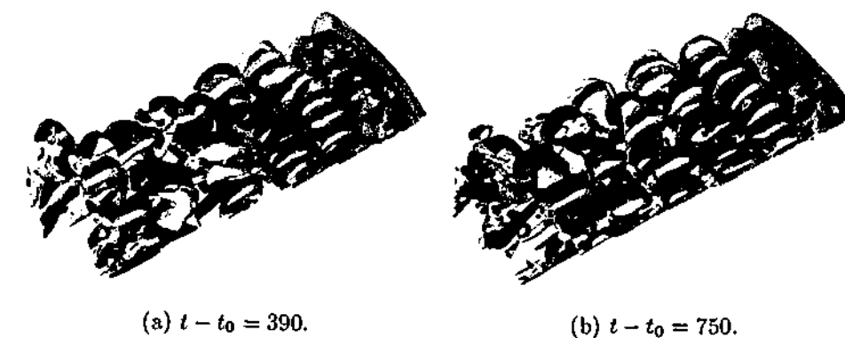
FIGURE 6.35: Isosurface plots of the saturated wake structures in the flow past a ring with Ar = 20 at Re = 320 . The azimuthal domain size is \lambda_{da} = 2L_0 , and contour shading is as per figure 6.8.
