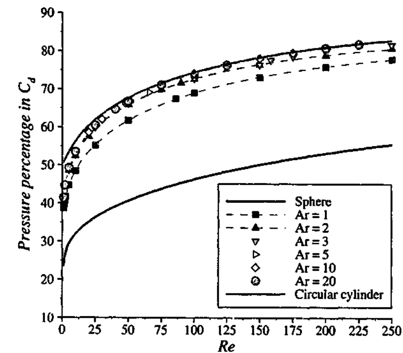
FIGURE 3.17: Percentage contribution of C_{dp} to C_d varying with Reynolds number for various rings. Symbols and colours are as per figure 3.13.
