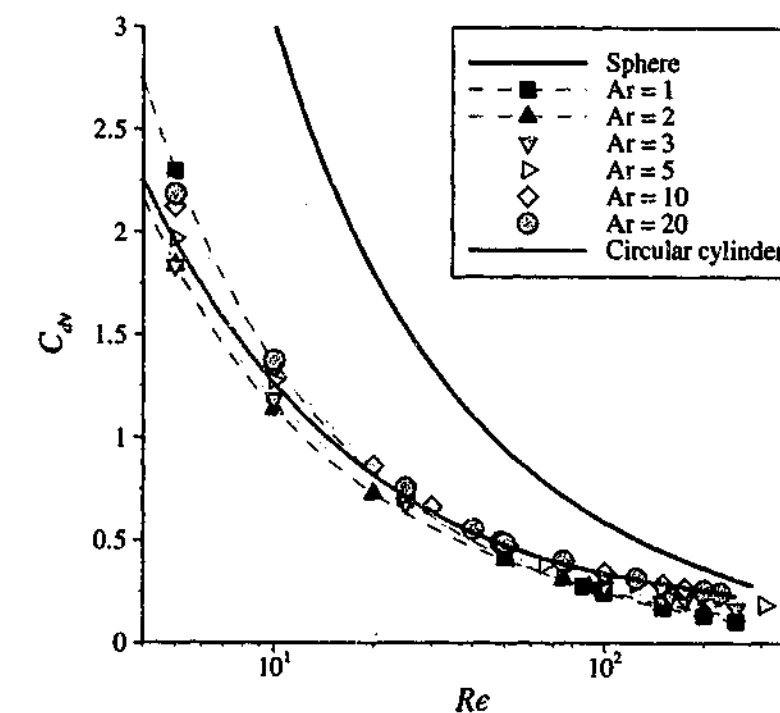
(b) Viscous drag component, C_{dv} .
