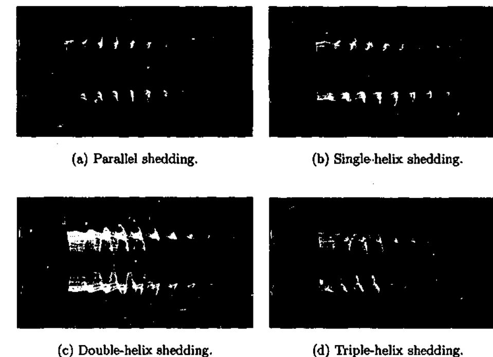
FIGURE 1.8: Vortex-shedding modes in the wake behind a ring with Ar = 24.3 at Re = 105 (from Leweke & Provansal 1995). The modes were identified by observing the deformation of a cylindrical smoke sheet.
