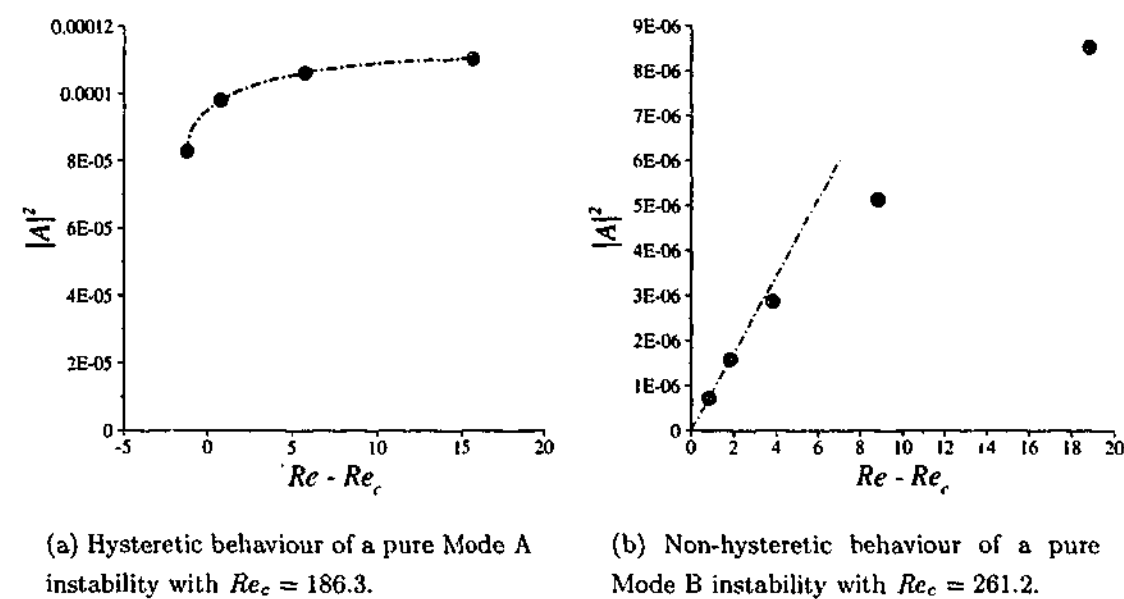
FIGURE 5.33: Plots of |A|^2 with Re - Re_c in the vicinity of the transitions for both the pure Mode A (a) and Mode B (b) instabilities in the wake behind a ring with Ar = 20 . The dots represent the measured amplitudes, and the lines provide approximate fits to the data.
