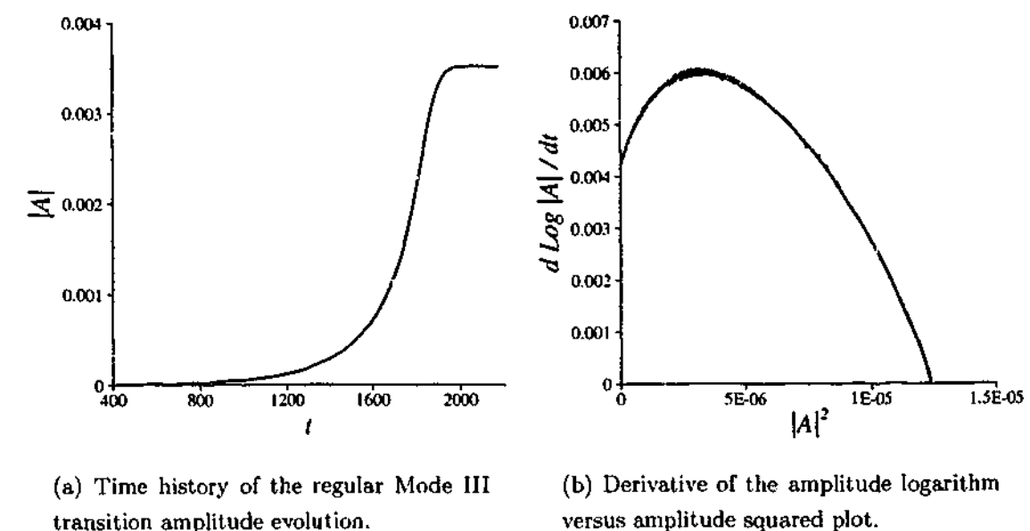
FIGURE 5.13: Plots used to determine the coefficients of the Landau model for the regular Mode III transition in the flow past a ring with Ar = 2 at Re = 93 . In (b), the non-linear profile and positive slope near the y -axis indicate that the transition is subcritical.
