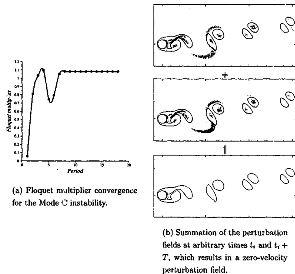
FIGURE 4.9: Verification that the Mode C instability is subharmonic. In (a), the convergence of the Floquet multiplier suggests that the mode has no imaginary component, and in (b), the perturbation field is observed to alternate in sign from one period to the next.
