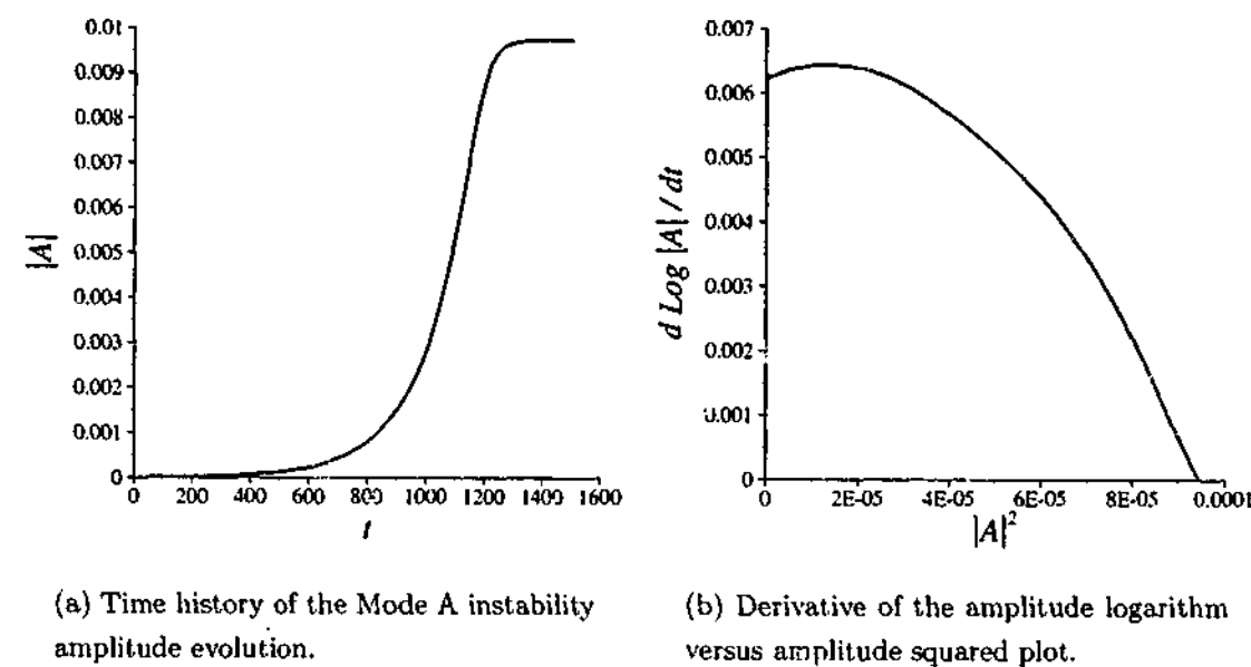
FIGURE 5.25: Plots used to determine the coefficients of the Landau model for the Mode A transition in the flow past a ring with Ar = 10 at Re = 200 . In (b), the non-linear profile and positive slope near the y -axis indicate that the transition is subcritical.
