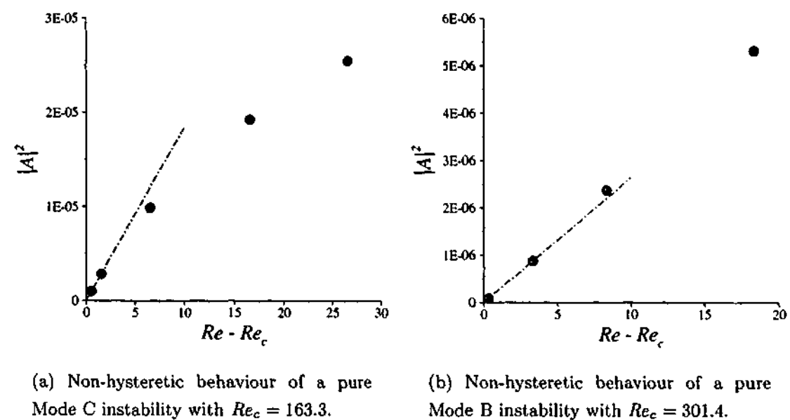
FIGURE 5.20: Plots of |A|^2 with Re - Re_c in the vicinity of the transitions for both the pure Mode C (a) and Mode B (b) instabilities in the wake behind a ring with Ar = 5 . The dots represent the measured amplitudes, and the lines provide a linear fit to the data through Re - Re_c = 0 .
