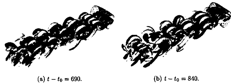
FIGURE 6.22: Isosurface plots of the saturated wake structures in the flow past a ring with Ar = 20 at Re = 280 , with the Mode C wavelengths dominating the wake (a), and where Mode A, Mode B and Mode C contribute a similar amount of energy to the wake (b). The azimuthal domain size and contour shading are as per figure 6.8.
