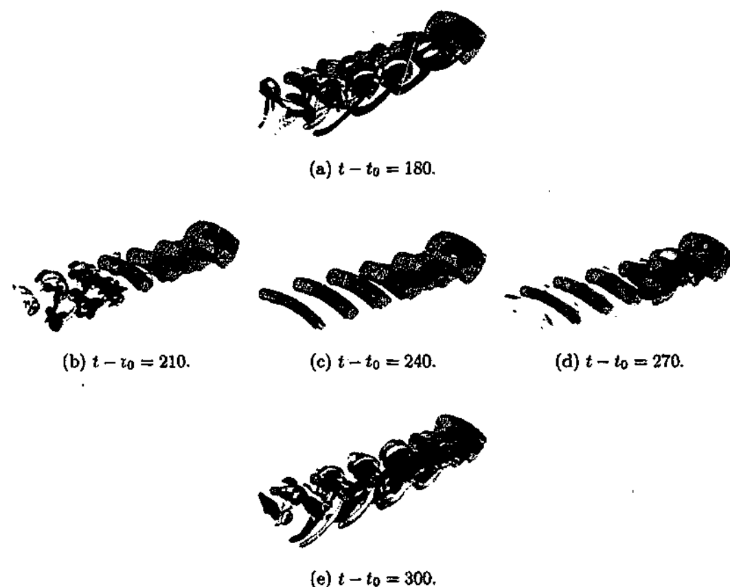
FIGURE 6.13: Isosurface plots of the saturated wake structures in the flow past a ring with Ar = 10 at Re = 240 , at several times throughout the computation. The azimuthal domain size and contour shading are as per figure 6.8.
