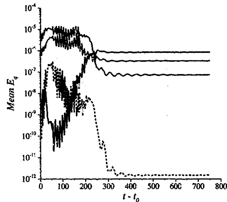
FIGURE 6.4: Evolution of the mean kinetic energy per period ( E_q ) for each azimuthal mode in the flow past a ring Ar = 5 with Re = 220 . Axes and lines are as per figure 6.1.
