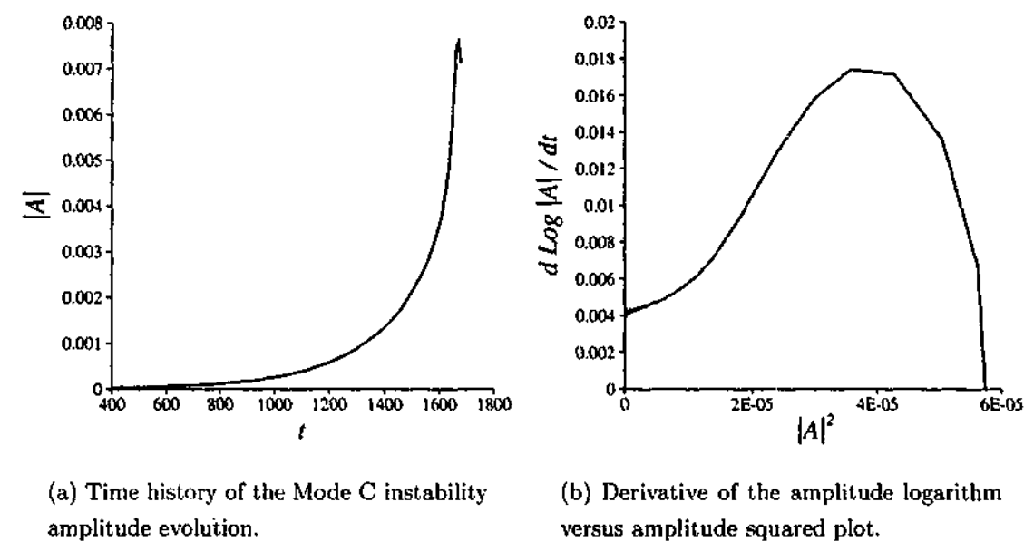
FIGURE 5.27: Plots used to determine the coefficients of the Landau model for the Mode C transition in the flow past a ring with Ar = 10 at Re = 230 . In (b), the non-linear profile and positive slope near the y -axis indicate that the transition is subcritical.
