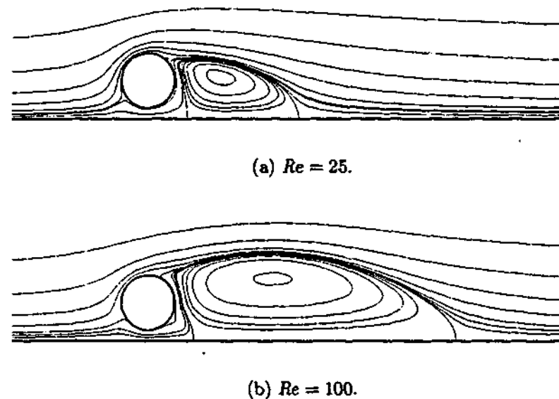
FIGURE 3.4: Flow streamlines around a ring with aspect ratio Ar = 1.4 . In (a) the axial recirculation bubble located downstream of the ring is observed. In (b), this bubble is significantly larger, and a divergence of streamlines from the lower right surface of the ring cross-section may be observed, corresponding to boundary layer separation. Again, the contour levels of the streamline plots are arbitrary.
