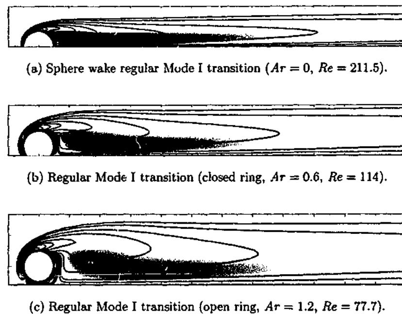
FIGURE 4.6: Plots of the base flow vorticity (arbitrary blue contour lines), and the streamwise vorticity of the perturbation field (red negative and green positive vorticity) of the primary instability for rings with 0 \leq Ar \leq 3 .
