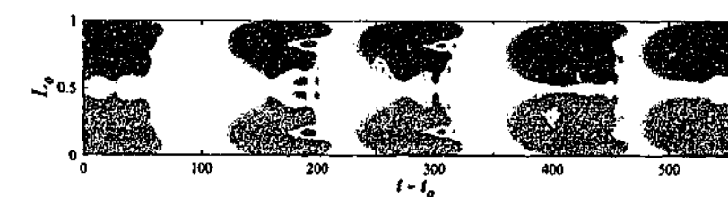
(b) Re = 240 .
