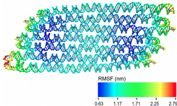
Mean structure/flexibility analysis
