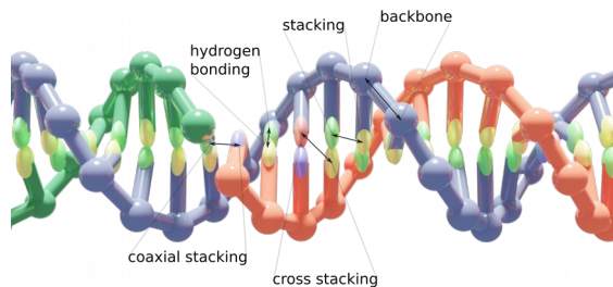
OxDNA: coarse-grained model for nucleic acid nanotechnology
