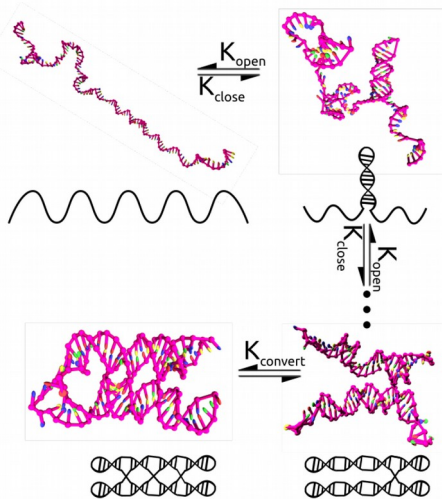
RNA tile folding pathway
