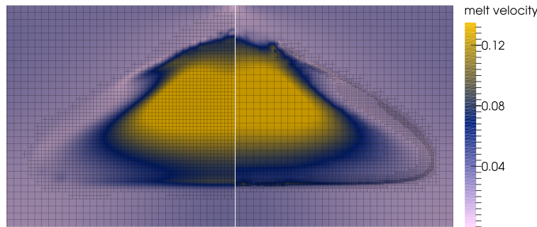
Figure 65: Mesh after a time of 3.6 million years for a model using the composition threshold refinement strategy (left) and the compaction length refinement strategy (right). Background colors indicate the melt velocity. Its sharp gradients at the interface between regions with and without melt can only be resolved using the compaction length refinement strategy.
