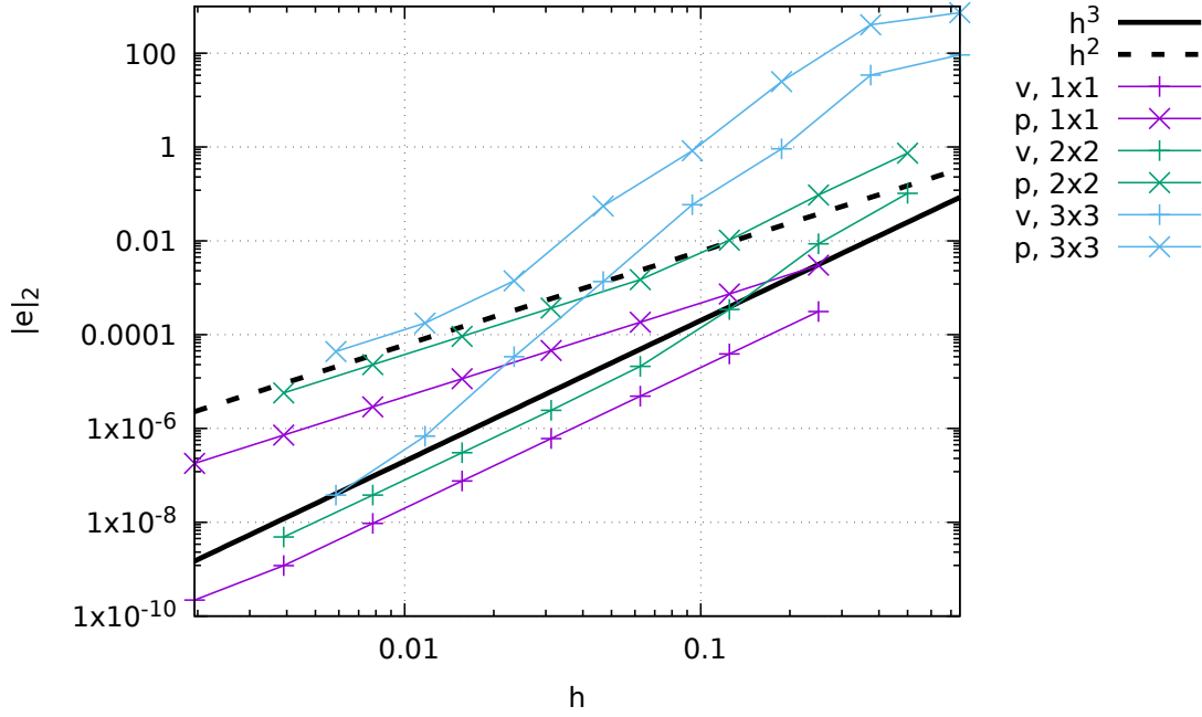
Figure 99: Viscosity grooves benchmark: Velocity and pressure error convergence as a function of the mesh size h for 3 domain sizes.
