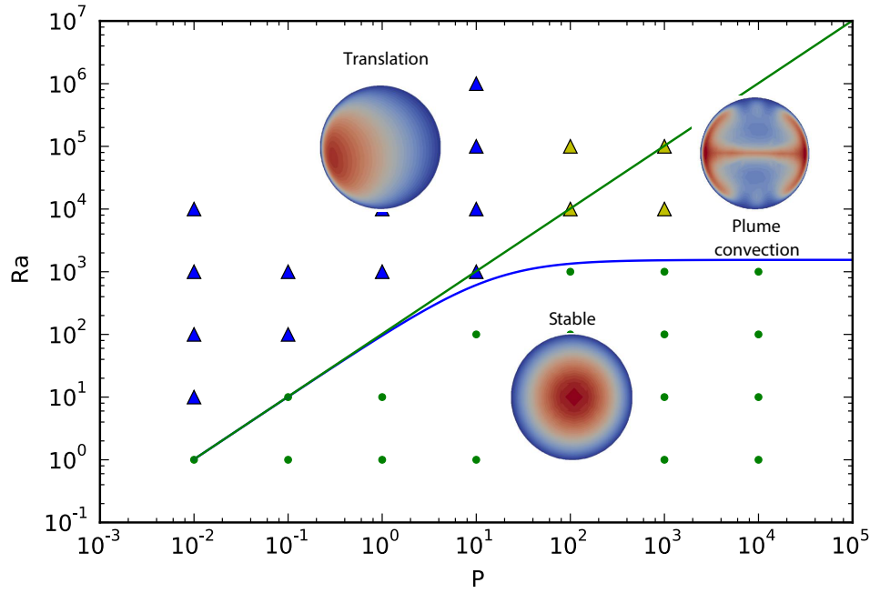
Figure 59: Stability diagram for convection in a sphere with phase change at its outer boundary. The stability curves for the first unstable mode ( l=1 ) and the translation are obtained from [28]. Each dot (no convection) and triangle (blue: translation, yellow: plume convection) is one model run done with ASPECT. The highest the Ra and P are, the more refinement is required (see text).
