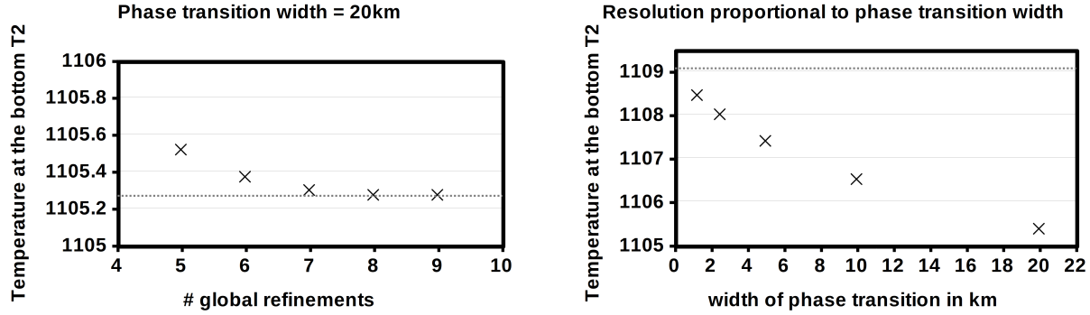
Figure 101: Results of the latent heat benchmark. Both figures show the modelled temperature T_2 at the bottom of the model domain. Left: T_2 in dependence of resolution using a constant phase transition width of 20 km. With an increasing number of global refinements of the mesh, the bottom temperature converges against a value of T_2 = 1105.27 K. Right: T_2 in dependence of phase transition width. The model resolution is chosen proportional to the phase transition width, starting with 5 global refinements for a width of 20 km. With decreasing phase transition width, T_2 approaches the theoretical value of 1109.08 K
