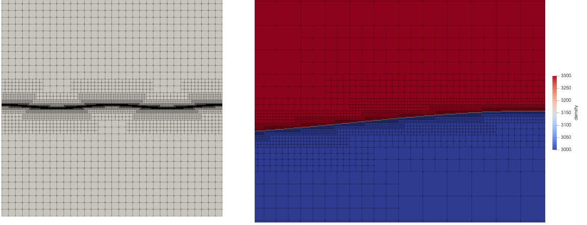
Figure 77: Left: grid with initial global refinement 4 and adaptive refinement 6; Right: density field with detail of the mesh.
