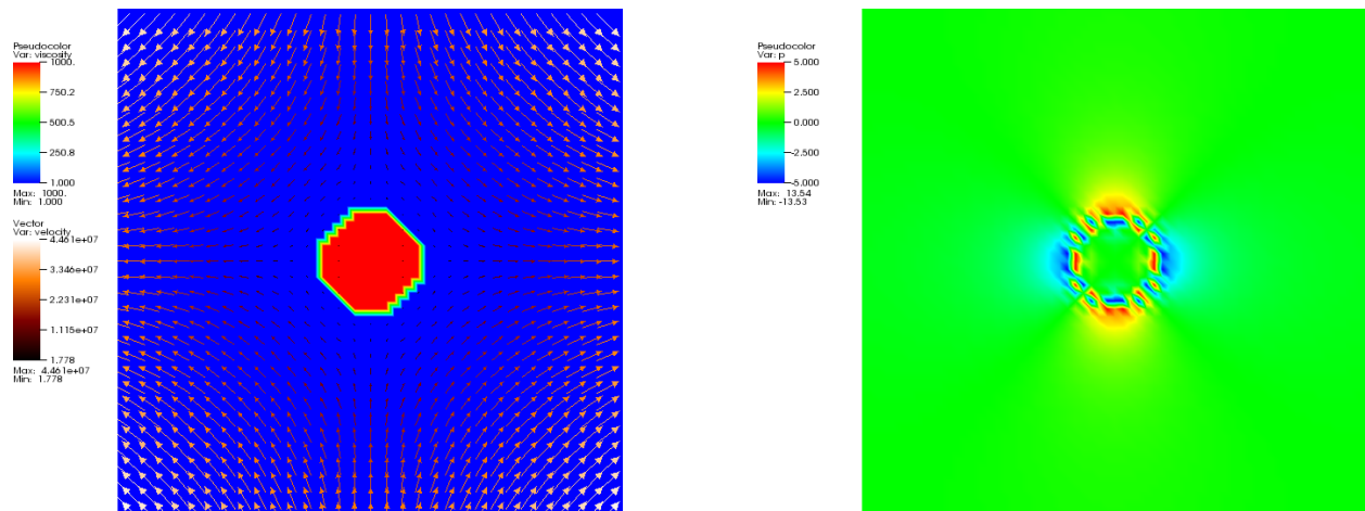
Figure 86: Inclusion Stokes benchmark. Left: The viscosity field when interpolated onto the mesh (internally, the “exact” viscosity field – large inside a circle, small outside – is used), and overlaid to it some velocity vectors. Right: The pressure with its oscillations along the interface. The oscillations become more localized as the mesh is refined.
