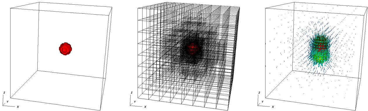
Figure 96: Stokes benchmark. Three-dimensional views of the compositional field (left), the adaptively refined mesh (center) and the resulting velocity field (right).
