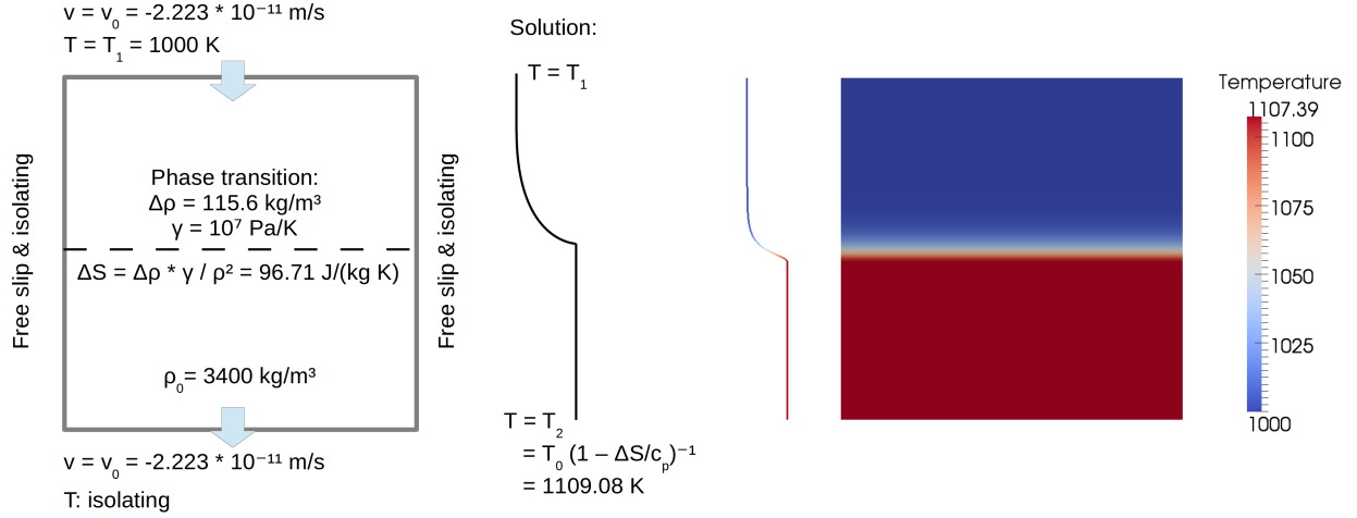
Figure 100: Latent heat benchmark. Both figures show the 2D box model domain. Left: Setup of the benchmark together with a sketch of the expected temperature profile across the phase transition. The dashed line marks the phase transition. Material flows in with a prescribed temperature and velocity at the top, crosses the phase transition in the center and flows out at the bottom. The predicted bottom temperature is T_2 = 1109.08 K. Right: Temperature distribution of the model together with the associated temperature profile across the phase transition. The modelled bottom temperature is T_2 = 1107.39 K.
