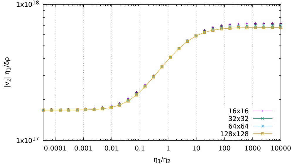
Figure 82: Scaled velocity measurements as a function of the viscosity contrast between surrounding medium and block for all experiments.
