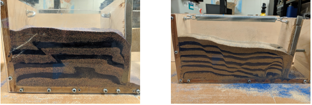
Figure 119: Examples of deformation patterns of “sand box” experiments in which alternating layers of differently-colored sand undergo deformation. Pictures courtesy of the lab of Dennis Harry at Colorado State University.
