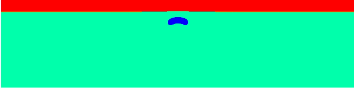
Figure 106: Setup for the dynamic topography benchmark. Again, the domain is 2800 km wide and 700 km high. A 100 km thick lid with viscosity 10^{23} overlies a mantle with viscosity 10^{21} . Both the lid and the mantle have a density of 3300 \text{ kg/m}^3 . A blob with diameter 100 km lies 300 km from the bottom of the domain. The blob has a density of 3200 \text{ kg/m}^3 and a viscosity of 10^{20} \text{ Pa s} .
