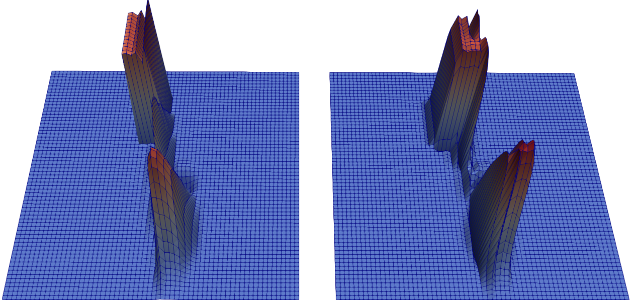
Figure 116: Dropping box benchmark at final time. Left: entropy viscosity. Right: SUPG.
