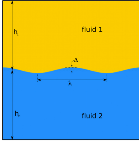
Figure 76: Setup of the Rayleigh-Taylor instability benchmark (taken from [85])
