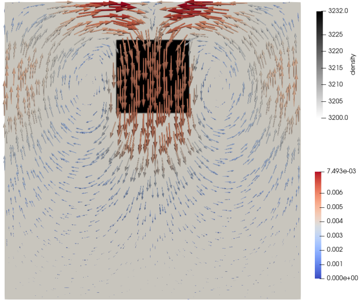
Figure 81: Density field with velocity arrows for \eta_2 = 10^{27} Pa s and \delta\rho = 32\text{kg/m}^3
