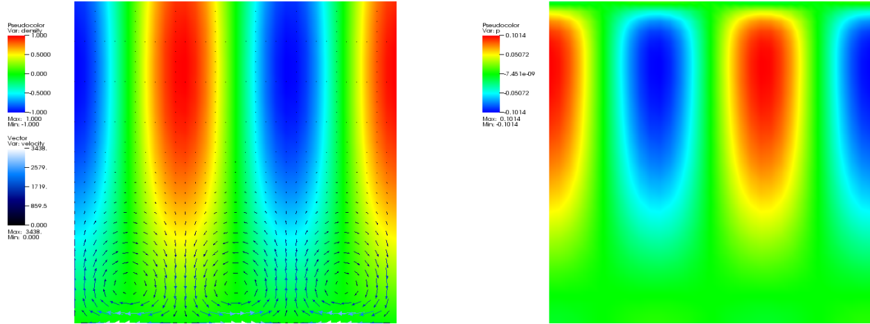
Figure 84: SolKz Stokes benchmark. Left: The density perturbation field overlaid with velocity vectors. The viscosity grows exponentially in the vertical direction, leading to small velocities at the top despite the large density variations. Right: The pressure.
