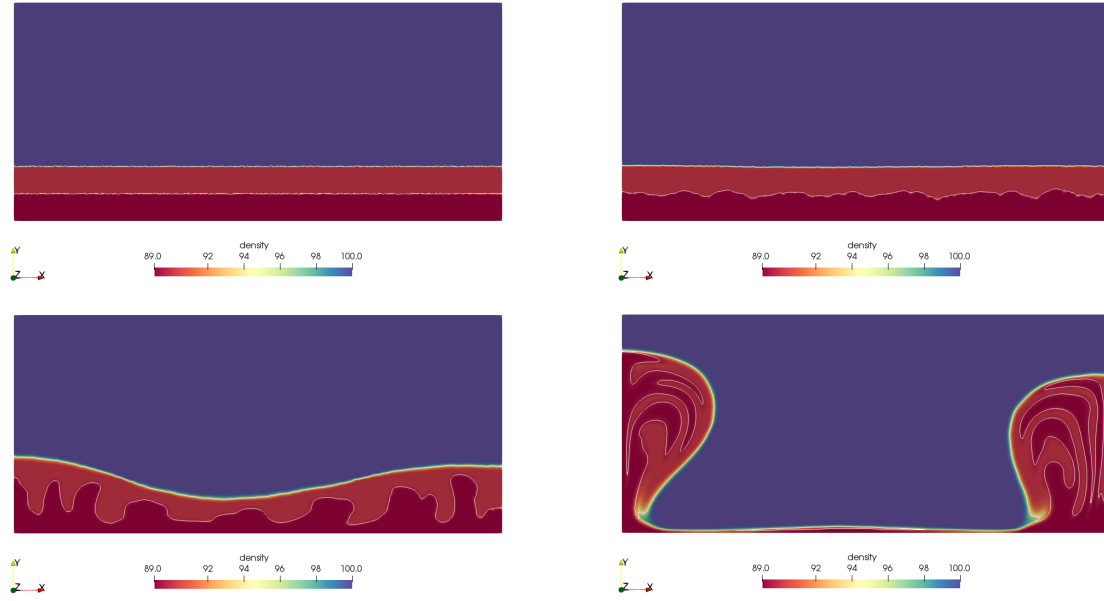
Figure 79: Polydiapirism benchmark: Density field at t = 0, 25, 50, 75 s.
