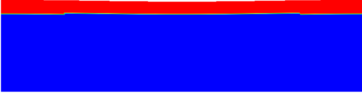
Figure 104: Setup for the topography relaxation benchmark. The box is 2800 km wide and 700 km high, with a 100 km lid on top. The lid has a viscosity of 10^{23} Pa s, while the mantle has a viscosity of 10^{21} Pa s. The sides are free slip, the bottom is no slip, and the top is a free surface. Both the lid and the mantle have a density of 3300 \text{ kg/m}^3 , and gravity is 10 \text{ m/s}^2 . There is a 7 km sinusoidal initial topography on the free surface.
