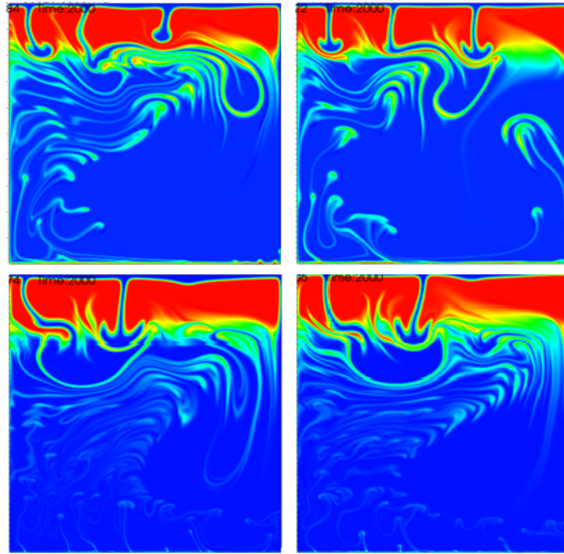
Figure 74: Van Keken benchmark two-layer viscosity model at final time step number, t = 2000 . These images show layers of different compositions and viscosities. Discontinuous cases are the left images, smooth cases are the right. The upper images are \frac{\eta_t}{\eta_b} = 0.1 , and the lower are \frac{\eta_t}{\eta_b} = 0.01 .
