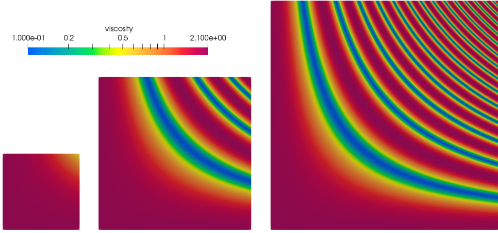
Figure 98: Viscosity grooves benchmark: Viscosity field for three domain sizes: 1 \times 1 , 2 \times 2 and 3 \times 3 .
