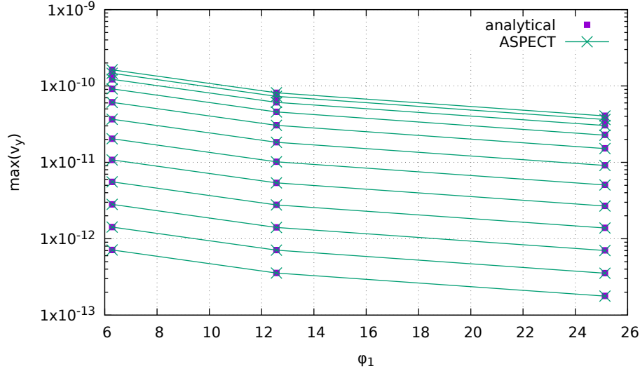
Figure 78: Maximum velocity for three values of the \phi_1 parameter.
