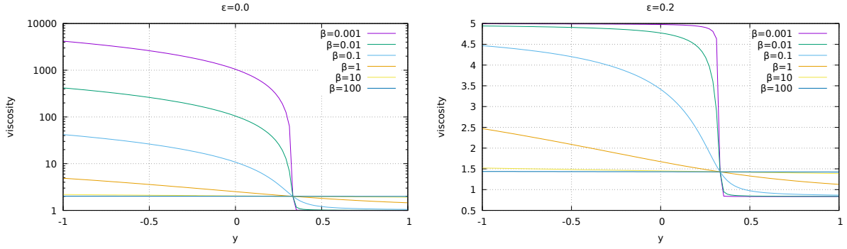
Figure 113: Layered flow benchmark: Viscosity profiles for various \beta values and two \epsilon values, using y_0 = 1/3 .
