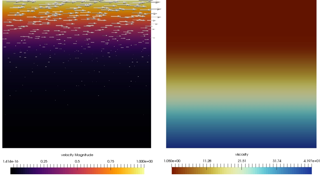
Figure 114: Velocity and viscosity fields for \beta = 0.01 and \epsilon = 0.05 at uniform level 8 resolution, using y_0 = 1/3 .
