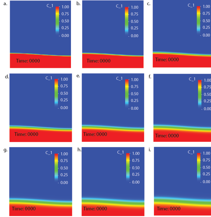
Figure 71: Van Keken Benchmark using smoothed out interface at 7 global refinements: compositional field at time t = 0 using smoothing parameter size: a) 0.0039, b) 0.0078, c) 0.0156, d) 0.0234, e) 0.0312, f) 0.0390, g) 0.0468, h) 0.0546, i) 0.0624.
