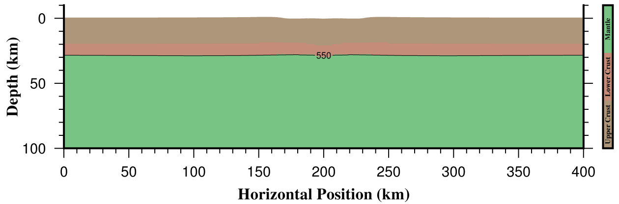
Figure 57: Compositional field after 5 \times 10^6 years of extension. The black line marks the 550\text{ }^{\circ}\text{C} isotherm.
