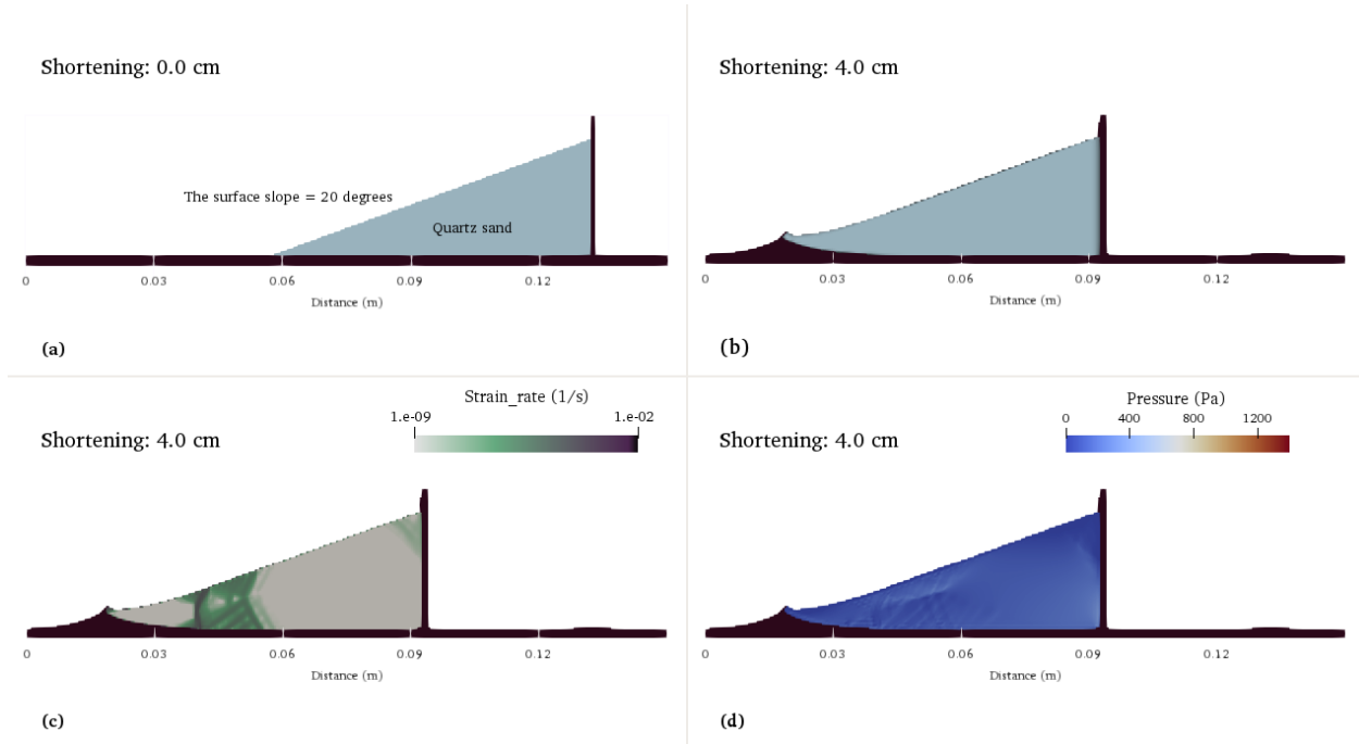
Figure 120: Numerical model of a stable sand wedge. a) Initial model setup. b) Material field after 4 cm of translation. c) Strain rate field and d) pressure field.
