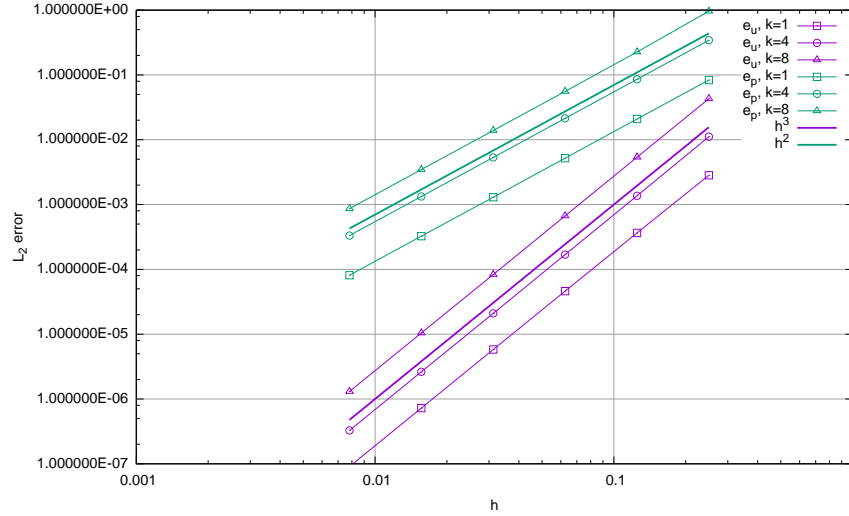
Figure 94: Velocity and pressure errors in the L_2 -norm as a function of the mesh size for the 2D annulus benchmark.
