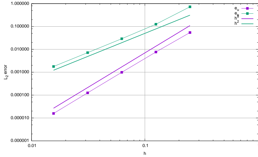
Figure 92: Velocity and pressure errors in the L_2 -norm as a function of the mesh size.
