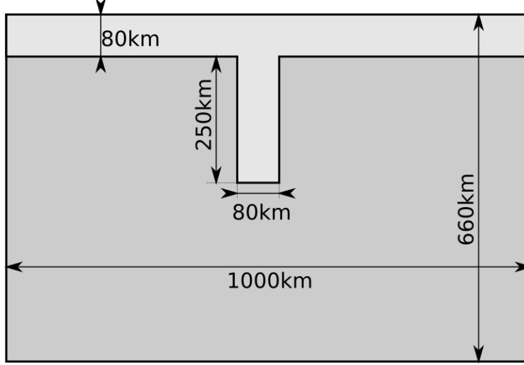
Figure 89: Slab detachment benchmark: Initial geometry
