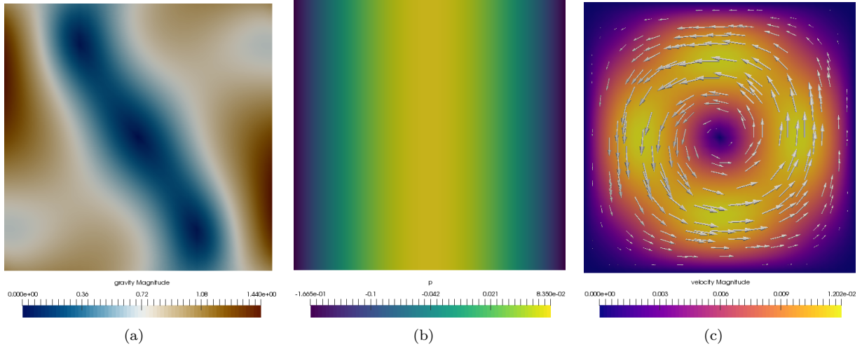
Figure 115: Donea & Huerta benchmark: Results for the 2D polynomial Stokes benchmark, obtained with a resolution of 32 \times 32 elements. (a) Gravity field, (b) pressure field, (c) velocity field.
