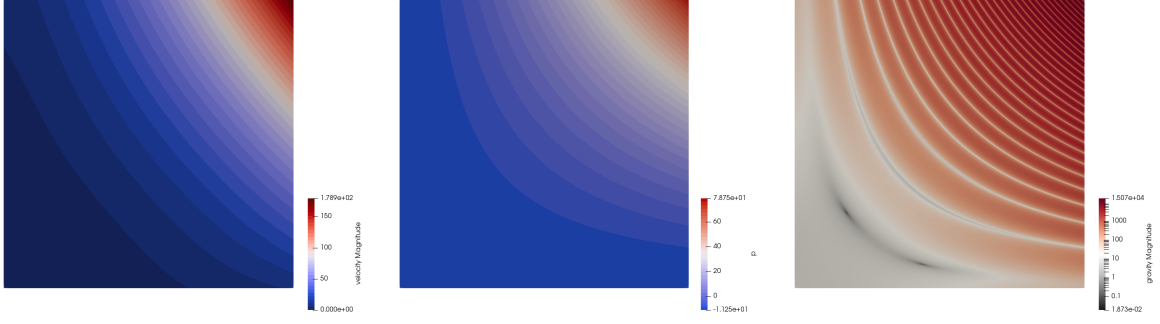
Figure 97: Viscosity grooves benchmark: From left to right, velocity field, pressure field, and norm of the right hand side of the momentum equation, for a 3 \times 3 domain with \epsilon = 0.1 .
