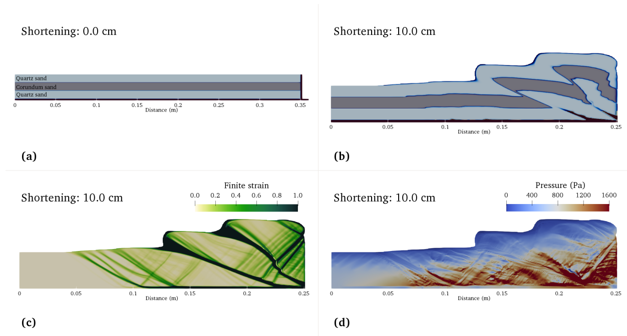
Figure 121: Numerical model of an unstable subcritical wedge. a) Initial model setup. b) Material field of sands after 10 cm shortening. c) Strain field and d) pressure field.
