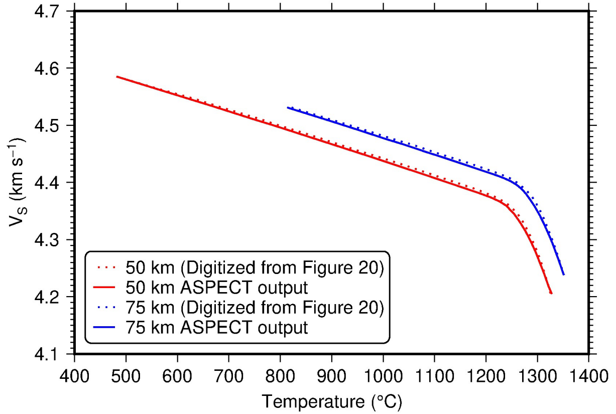
Figure 118: V_S as a function of temperature in the oceanic lithosphere. Dotted lines: digitized results from Fig. 20 of Yamauchi & Takei [97]; solid lines: ASPECT results; red = 50 km; blue = 75 km. Temperatures are taken from the plate model of McKenzie et al. [62] and V_S from the surface wave tomography model of Priestley et al. [67].
