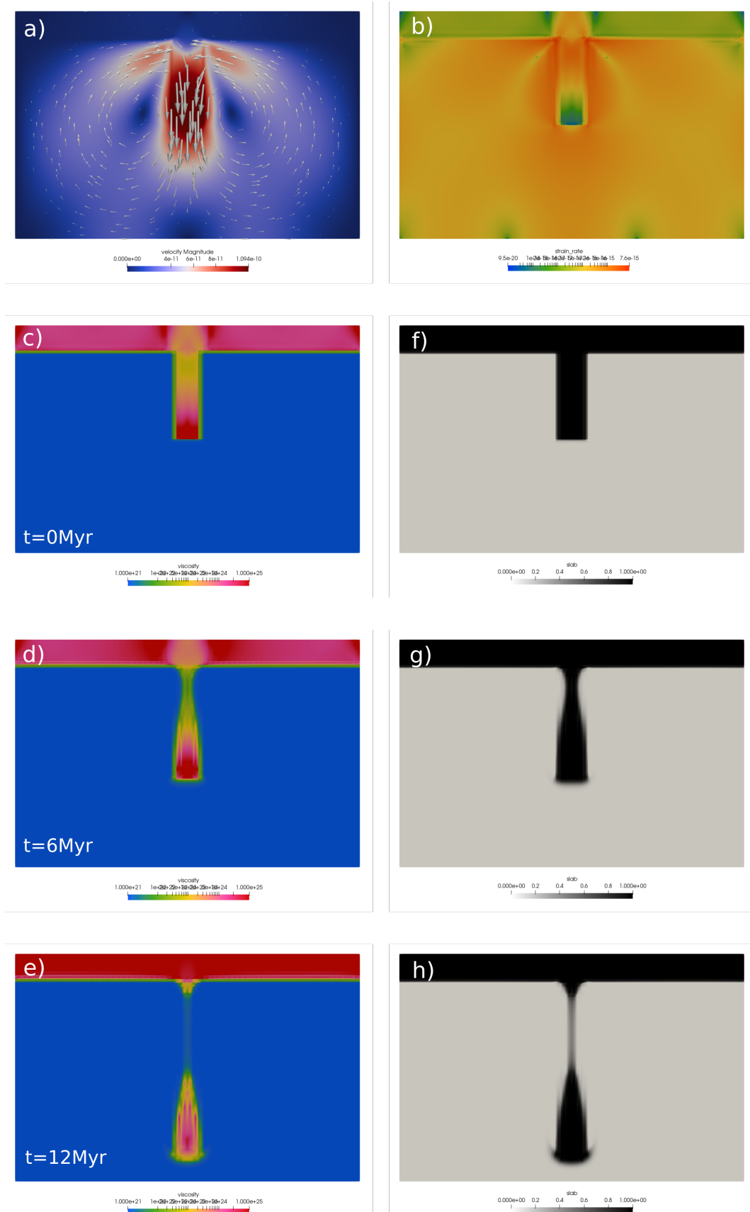
Figure 90: Slab detachment benchmark: a,b) velocity and strain rate fields at t = 0 . c,d,e) and f,g,h) time evolution of the viscosity and slab composition fields at t = 0, 6, 12\text{Myr} .
