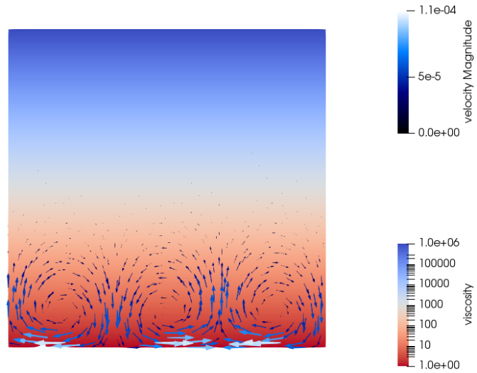
Figure 85: SolKz Stokes benchmark. Another view of the velocity vectors, this time plotted over the viscosity field.
