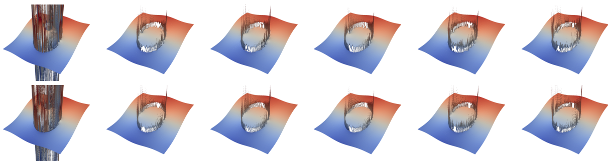
Figure 28: Visualization of the pressure field for the “sinker” problem. Like Fig. 27 but using the locally conservative, enriched Stokes element. Pressure values are shown in Table 3.
