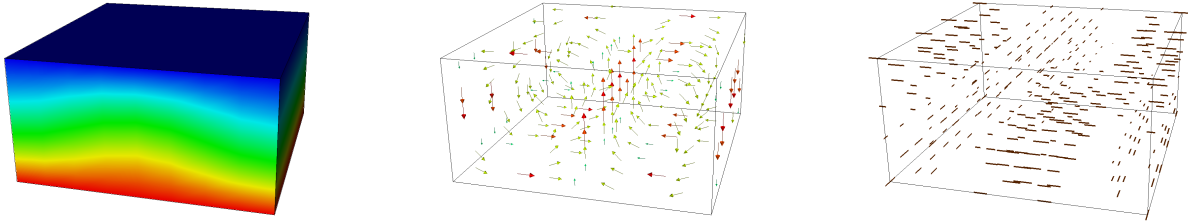
Figure 123: Illustration of the ‘maximum horizontal compressive stress’ visualization plugin. The left figure shows a ridge-like temperature anomaly. Together with no-slip boundary along all six boundaries, this results in two convection rolls (center). The maximal horizontal compressive strength at the bottom center of the domain is perpendicular to the ridge because the flow comes together there from the left and right, yielding a compressive force in left-right direction. At the top of the model, the flow separates outward, leading to a negative compressive stress in left-right direction; because there is no flow in front-back direction, the compressive strength in front-back direction is zero, making the along-ridge direction the dominant one. At the center of the convection rolls, both horizontal directions yield the same stress; the plugin therefore chooses an essentially arbitrary horizontal vector, but then uses a zero magnitude given that the difference between the maximal and minimal horizontal stress is zero at these points.
