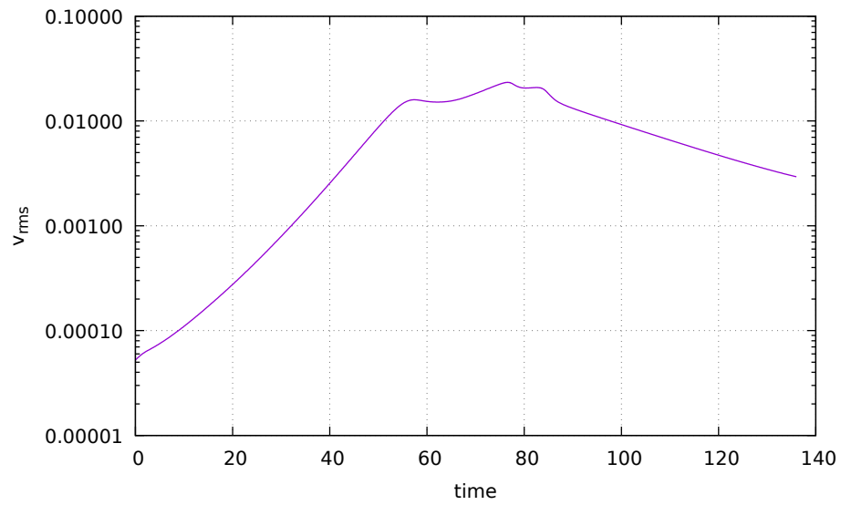
Figure 80: Polydiapirism benchmark: Root mean square velocity as a function of time
