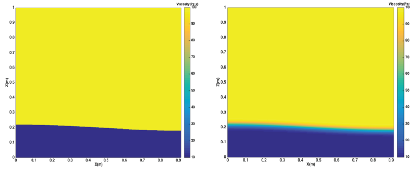
Figure 73: Van Keken benchmark using different-viscosity layers. The left image is the discontinuous case, while right is the smooth. Both are shown at t = 0 .
