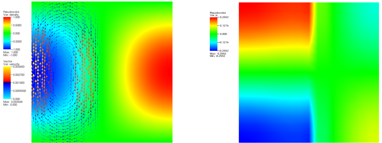
Figure 83: SolCx Stokes benchmark. Left: The density perturbation field and overlaid to it some velocity vectors. The viscosity is very large in the right hand, leading to a stagnant flow in this region. Right: The pressure on a relatively coarse mesh, showing the internal layer along the line where the viscosity jumps.
