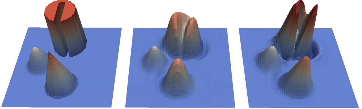
Figure 117: Rotating shapes benchmark at final time: Left: reference. Middle: Entropy viscosity. Right: SUPG.
