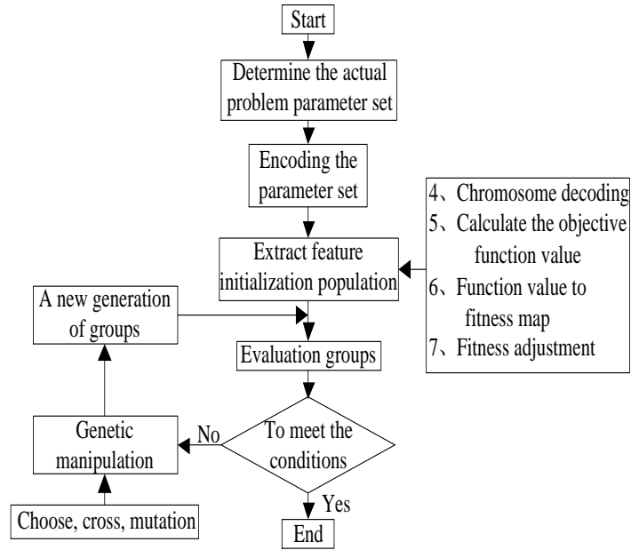
Figure 4 Flow chart of wireless sensor network abnormal vehicle load data recognition based on genetic algorithm
