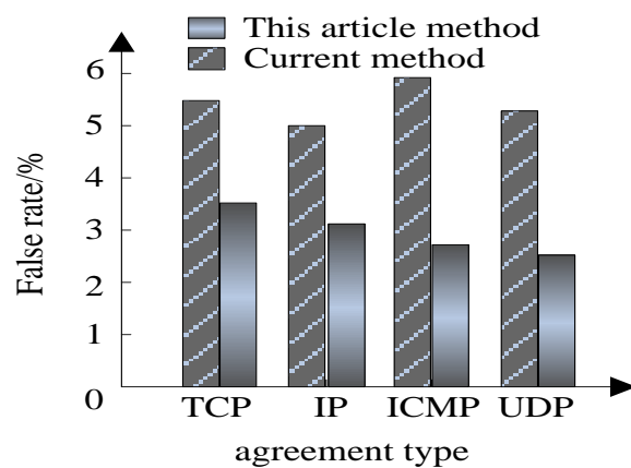
Figure 6 False recognition rate of two different methods
