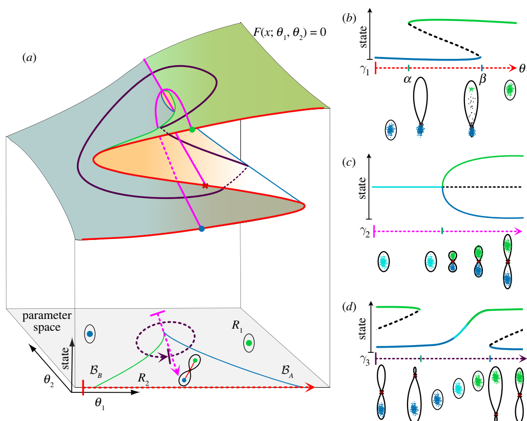
Figure 7. Bistability: the standard cusp. (a) Catastrophe manifold and bifurcation set. In 2D parameter space, the blue and green lines represent the bifurcation set with the colour of the line corresponding to the attractor involved in the fold bifurcation that occurs on that fold line. The dashed arrows indicate example paths in parameter space, corresponding to a continuous change in an extrinsic signal. The 2D catastrophe manifold on top of the parameter space shows the fold lines and the preimages of the different paths that are sketched with more detail in panels (b,c,d). In the region R_2 (inside the cusp, with three sheets above), there are two attractors A and B separated by a saddle S . When the parameters move out of R_2 to R_1 (outside the cusp, with one sheet above) by crossing \mathcal{B}_A (respectively, \mathcal{B}_B ) the attractor A (respectively, B ) and the saddle undergo a fold bifurcation which destroys A (respectively, B ). Paths \gamma_1 across the cusp, \gamma_2 vertically through the cusp, and \gamma_3 around the cusp correspond to the hysteresis, pitchfork and cusp smooth swap diagrams (respectively). (b) Bifurcation diagram of a genetic switch. Change in the rest points of a bistable system, as a parameter \theta_1 changes. A single attractor (green) is present when \theta = 0 . When \theta_1 crosses the bifurcation point ( \alpha ), a saddle (dashed curve) and a new attractor (blue) appear. When the parameter crosses a second bifurcation point ( \beta ) the initial attractor (green) collides with the saddle and disappears causing the cells in it to transition to the available attractor (blue). The coexistence of both attractors between \alpha and \beta results in bistability and hysteresis. (c) Pitchfork . As a parameter changes along \gamma_2 , an initial attractor becomes a saddle point and two attractors appear at each side. The system is symmetric with respect to the saddle point. (d) Smooth state swap . The path \gamma_3 around the cusp shows how cells transition from A into B without a step-like switch. When the path crosses the bifurcation set, the bifurcating attractor is empty and hence no cells are forced to transition, instead, going around the cusp in R_1 changes the gene expression in a smooth continuous way.
