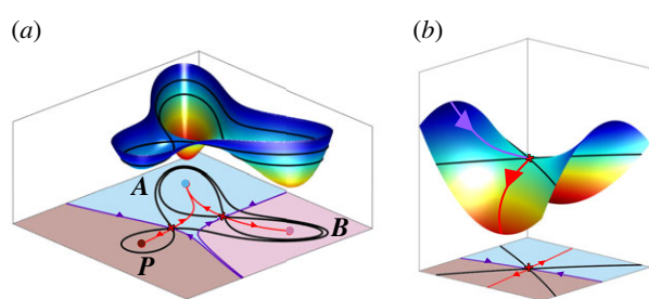
Figure 2. Two-dimensional landscapes. (a) System with three attractors and two saddles. The purple curves are the separatrices or stable manifolds of the saddles, the red curves are the unstable manifolds (if time is run backwards points on these converge to the saddle). Points on each unstable manifold converge to two attractors and the stable manifolds divide the phase space into three basins, one for each attractor. Level curves for the saddles are indicated in black. (b) Saddle point. The dynamics near a saddle point. The stable (purple) and unstable (red) manifolds are shown.
