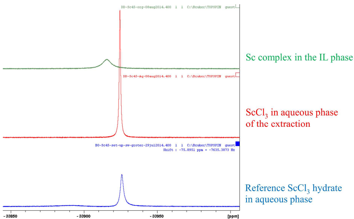
Figure S1. 45 Sc NMR spectra.
