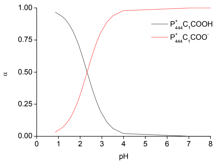
Figure S2. Fractional composition ( \alpha ) diagram of monoprotic acid P_{444}C_1COOH with pK_a = 2.32 .
