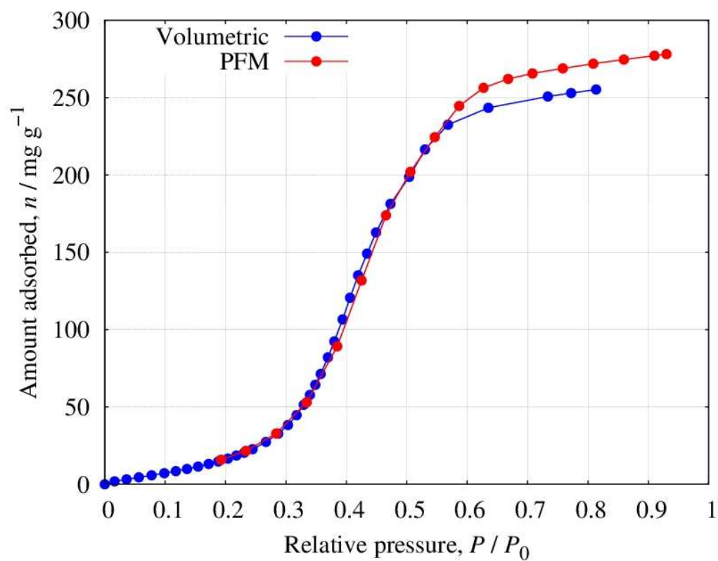
Figure S1. A comparison of water adsorption isotherms by PFM and volumetric method of A7 at 298 K. The isotherms show good agreement except high relative pressure region.
