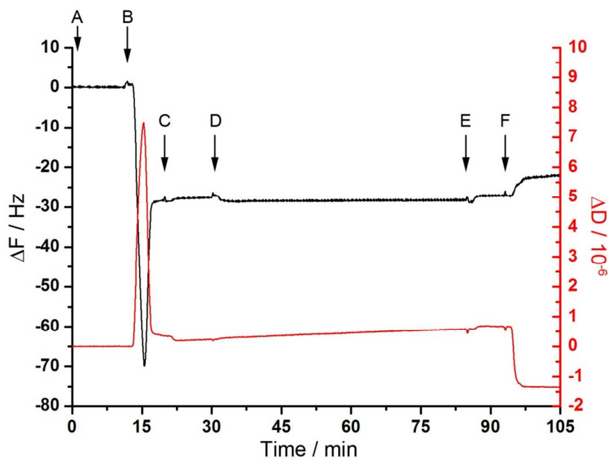
Fig. S1: No unspecific interaction of NERMAD on POPC/Chol/POPS (63:20:17)
