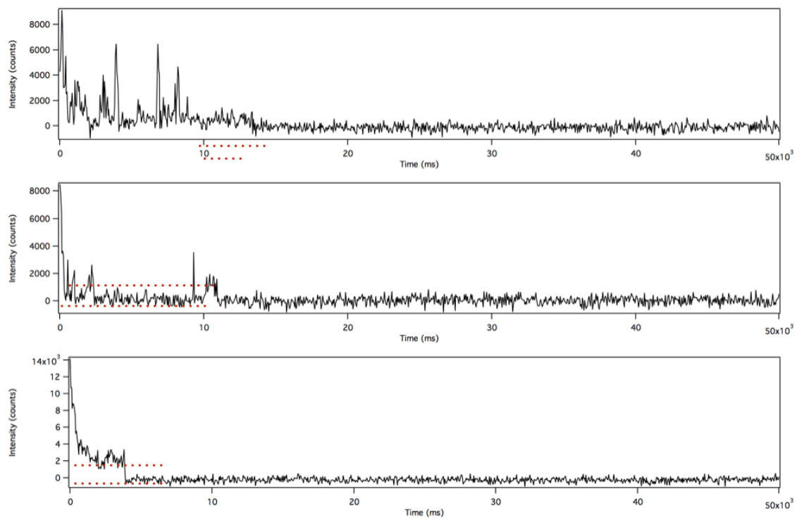
Figure SI-1. Typical decays with one step final bleaching
