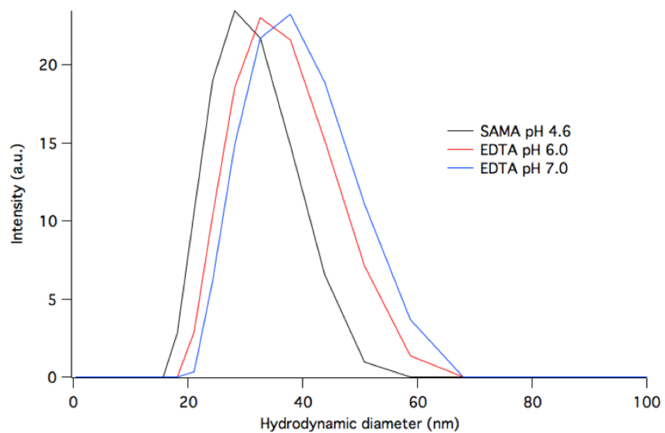
Figure SI-3. Dynamic light scattering showing expansion of BMV particles as the pH solution increases.
