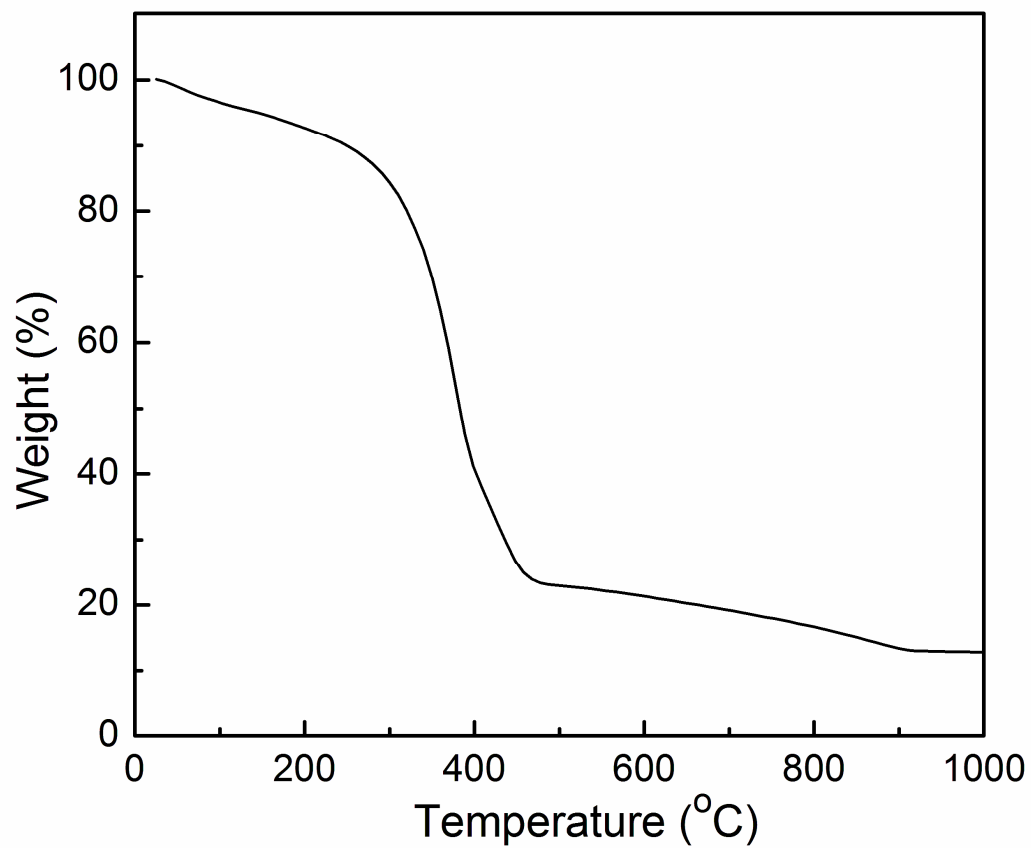
Figure S1. TGA curve of multi-component capsules. The final organic/inorganic weight percentage of capsules got from TGA is 6.8125 corresponding to a theoretical ratio 7.4708.
