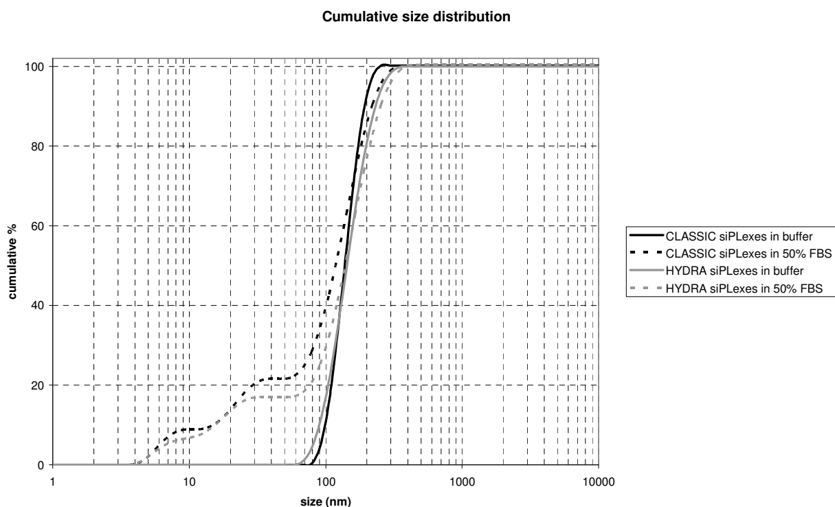
Figure S1. Cumulative size distribution of CLASSIC (black) and HYDRA (gray) siPLexes in absence (solid lines) and presence (dashed lines) of serum (FBS). SiPLexes were incubated for 1 hour at 37°C.
