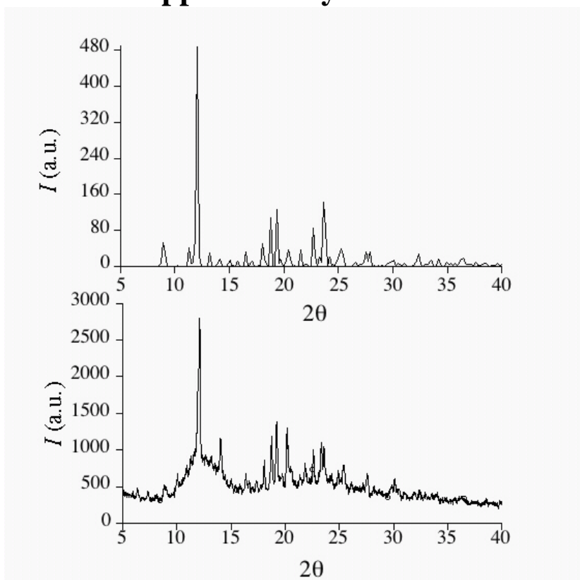
Figure S1. Experimental (After several months; bottom) and theoretical (top) powder pattern for [K(18\text{-crown-}6)][Mn(H_2O)_2Cr(ox)_3] \cdot 0.5(18\text{-crown-}6) ( 1 ).
