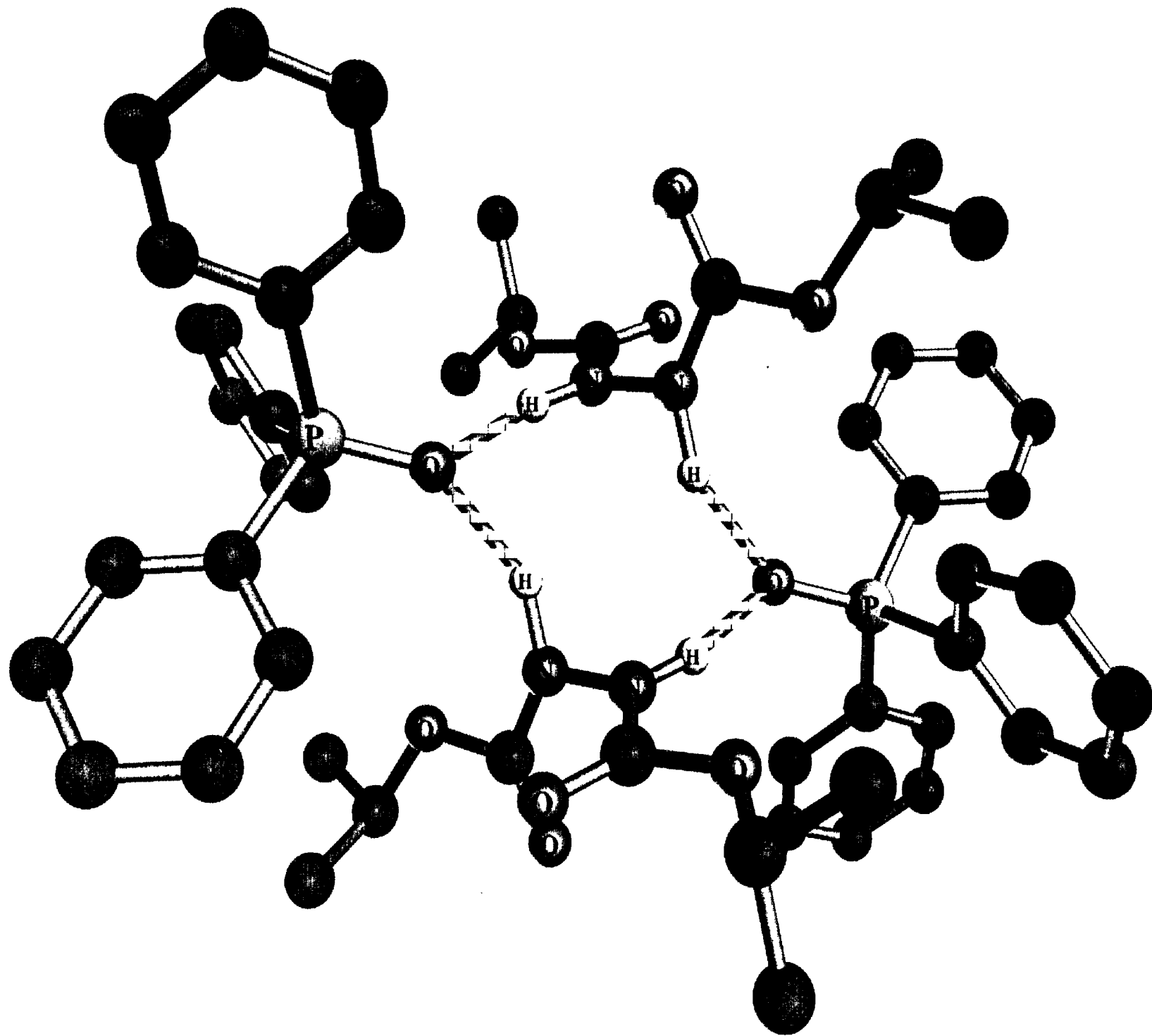
Triphenylphosphine oxide • diisopropyl hydrazinedicarboxylate
