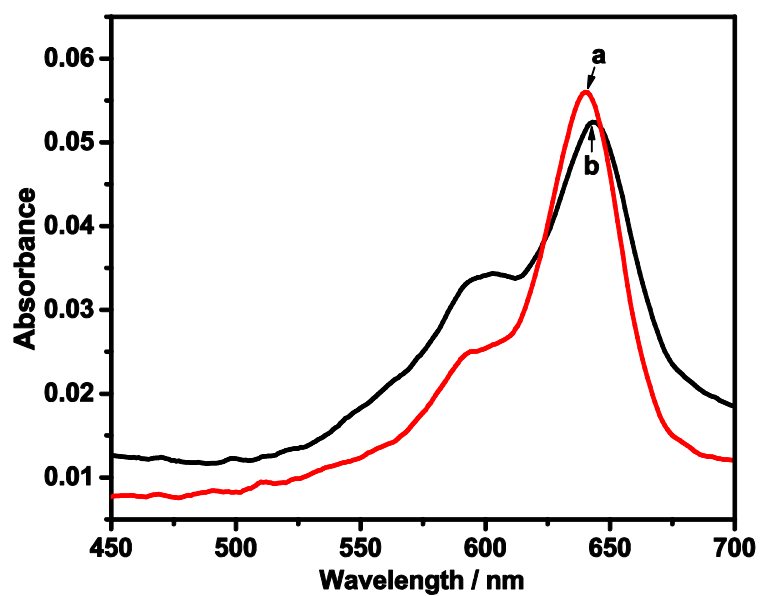
Figure S1. UV-Vis spectra of (a) Cy5-NHS, and (b) Cy5-penicillinase.
