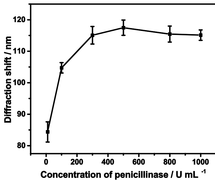
Figure S3. The diffraction shifts of activated CCH films pretreated with different concentrations of penicillinase in the presence of 5 mM penicillin G. The error bars indicate the standard deviation of three assays.
