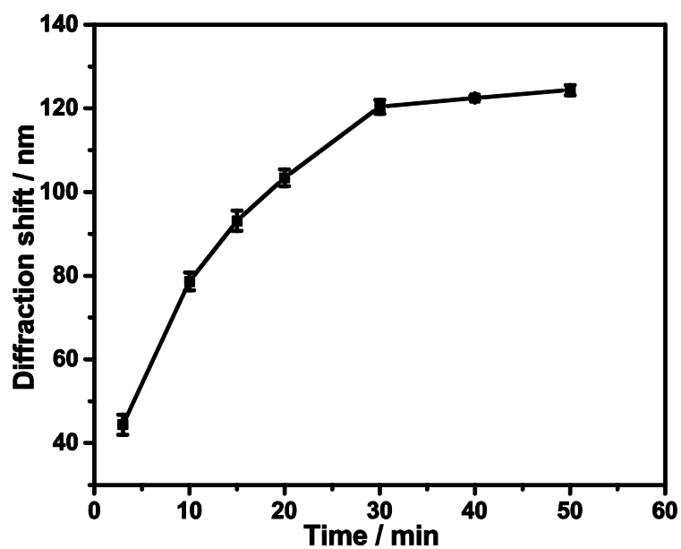
Figure S4. Effect of time on the diffraction shifts of PCCH film in the presence of 5 mM penicillin G. The error bars indicate the standard deviation of three assays.
