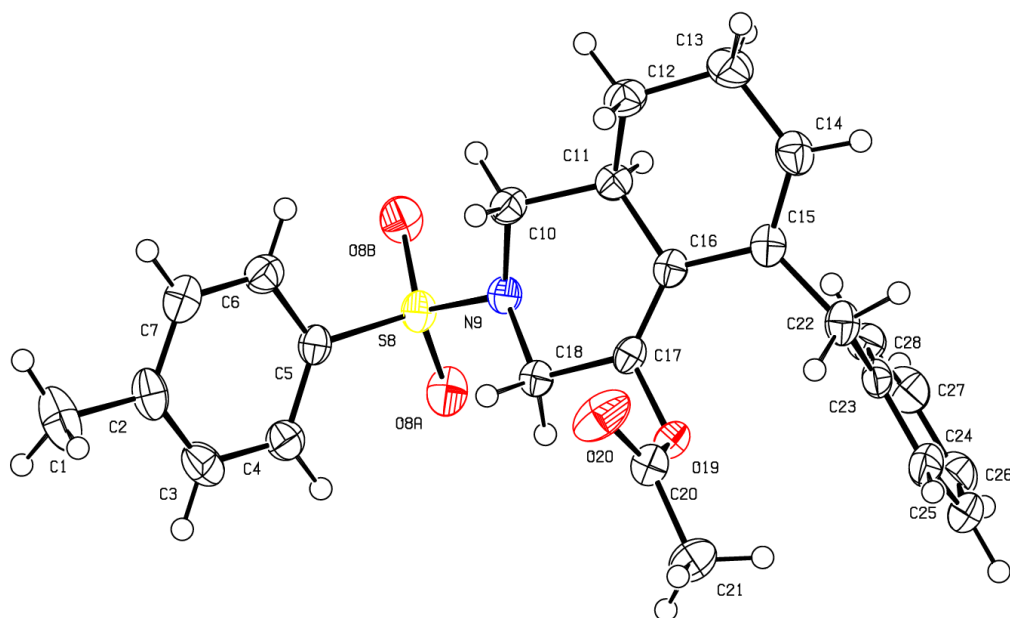
Figure S45. ORTEP Drawing of 3n with Thermal Ellipsoids at 50% Probability Levels S2
