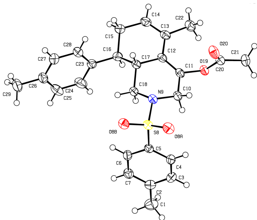
Figure S45. ORTEP Drawing of 3n with Thermal Ellipsoids at 50% Probability Levels S2
