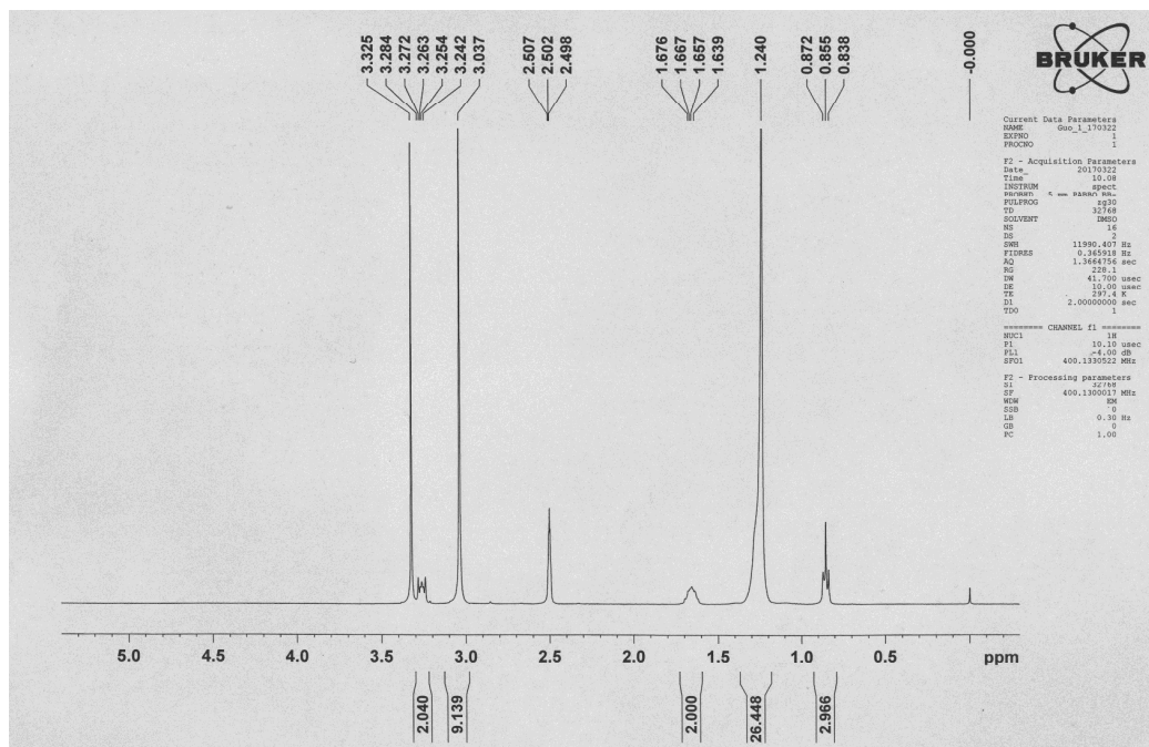
Figure S3. The ^1\text{H} NMR spectrum of CTAB.
