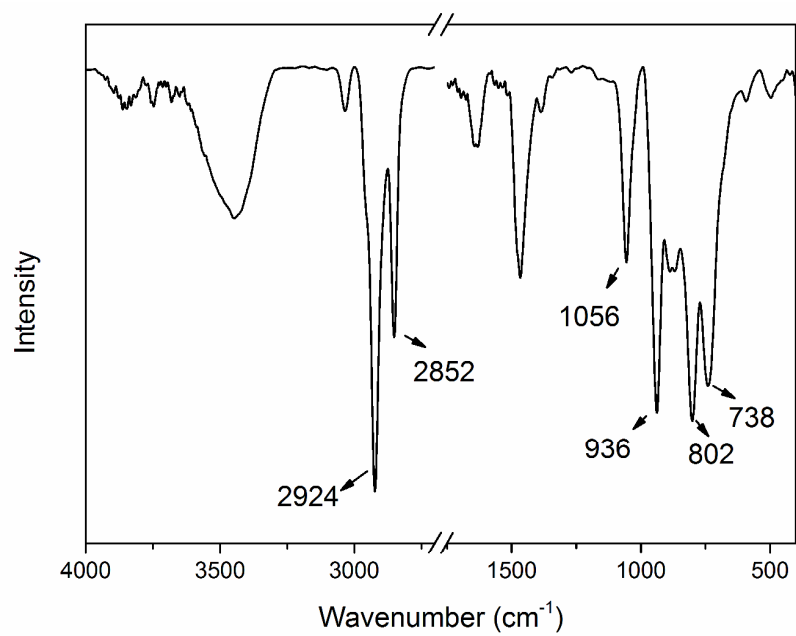
Figure S5. The FTIR spectrum of POM/CTAB hybrid solids.
