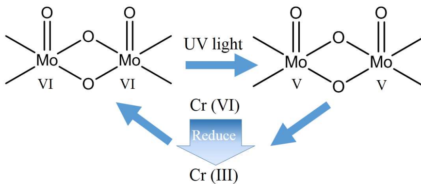
Figure S6. The schematic diagram of Cr (VI) degradation upon UV light irradiation by POM/CTAB.
