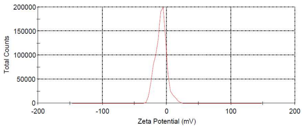
Figure S2. The Zeta potential curve of POM/CTAB hybrid materials solution.
