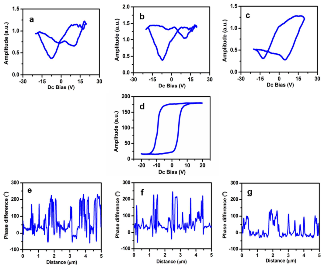
Fig. S3 Piezoelectric, ferroelectric responses and domain sizes of PSN-PMN-PT crystals (a, e: 0.1275PSN-0.3825PMN-0.49PT crystal; b, f: 0.27PSN-0.27PMN-0.46PT crystal; c, d, g: 0.39PSN-0.13PMN-0.48PT crystal)
